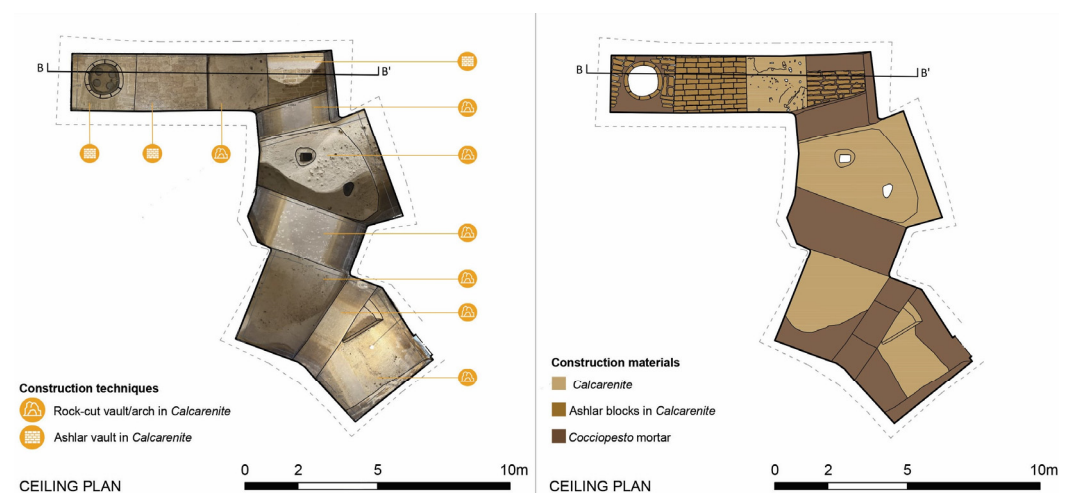
Figure 11. Materials and construction techniques of the vaulted system.
