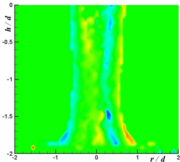
Fig 3C. Vorticity distribution of the annular jet without synthetic jet activation. Re = 1500 h/d = 2 .
