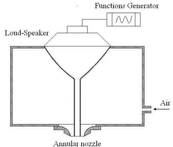
Fig. 2 Detail of the annular nozzle/synthetic jet arrangement.
