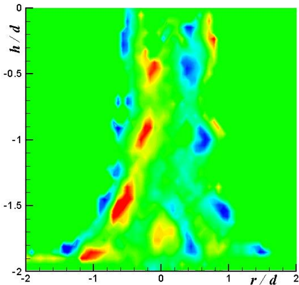
Fig. 5C Vorticity distribution at Re 1000, St 0.3 and h/d 2.
