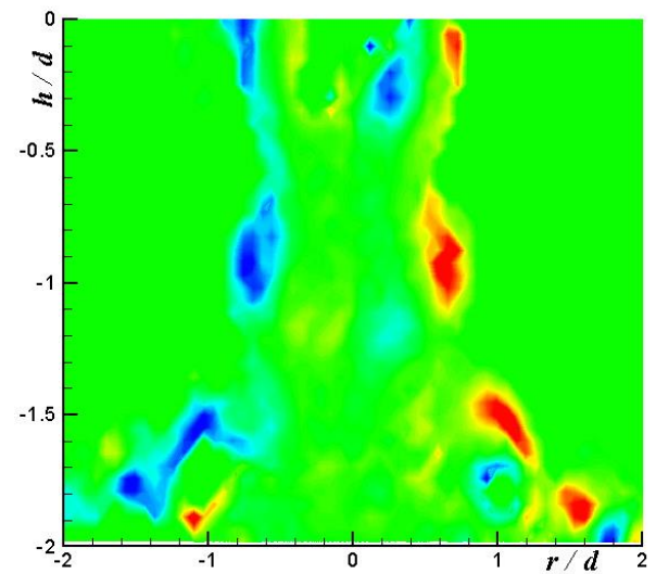
Fig. 4C Vorticity distribution at Re 1500; h/d = 2 ; synthetic jet oscillating at 212 Hz.
