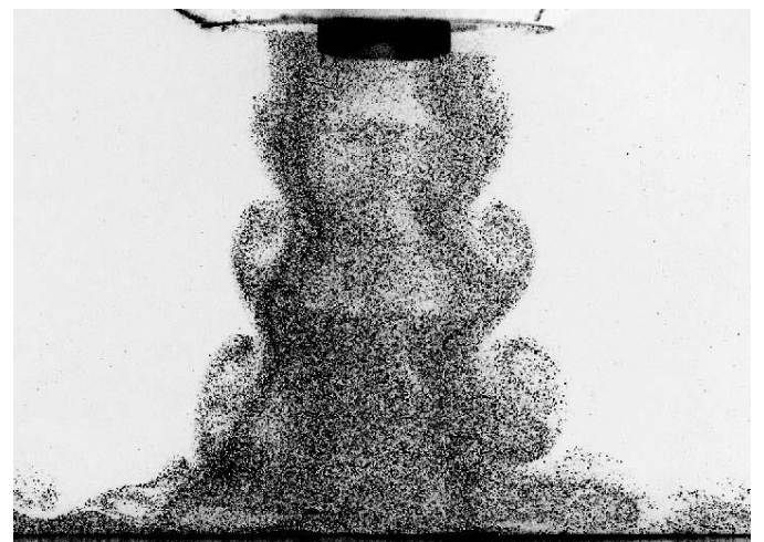
Fig. 5A. PIV image of annular jet at Re 1000, St = 0.3 , h/d = 2 .
