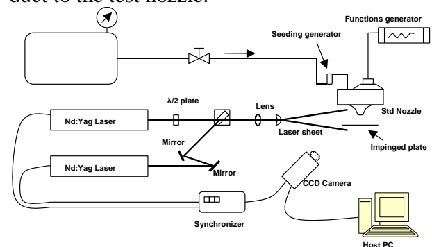
Fig. 1. PIV set-up and system components
