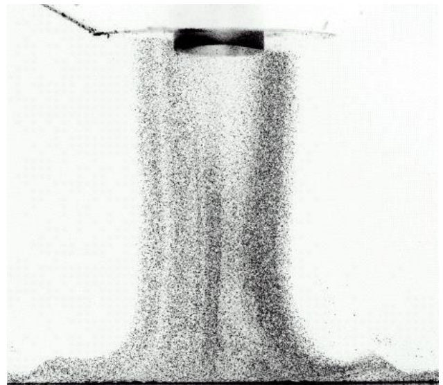
Fig 3A. PIV image of the annular jet without synthetic jet activation. Re = 1500 h/d = 2 .
