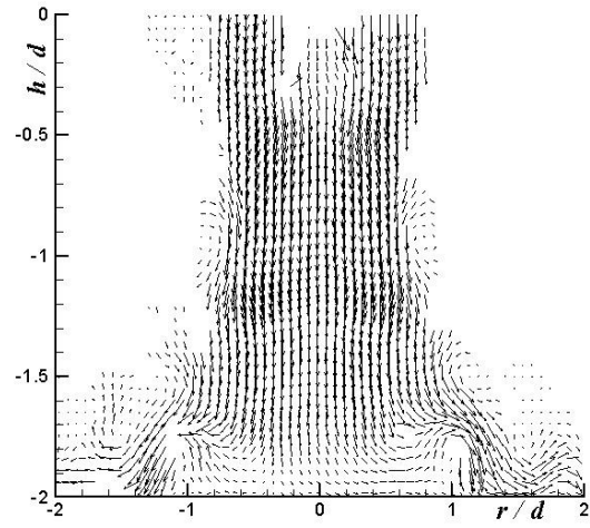
Fig 4B. PIV Velocity distribution at Re 1500, St = 0.3 , h/d = 2 .
