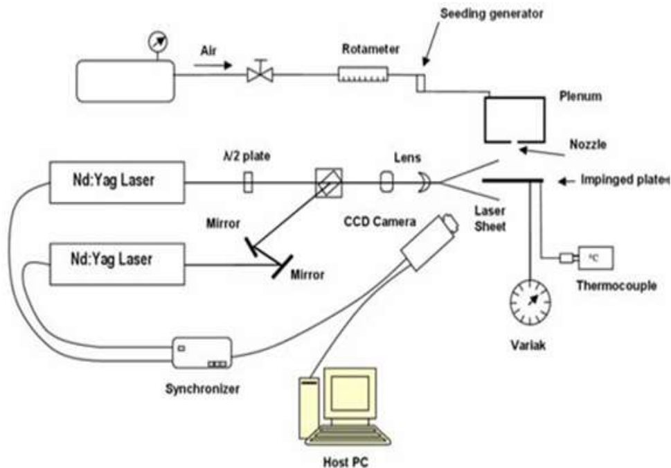
Fig. 1. Experimental set-up
