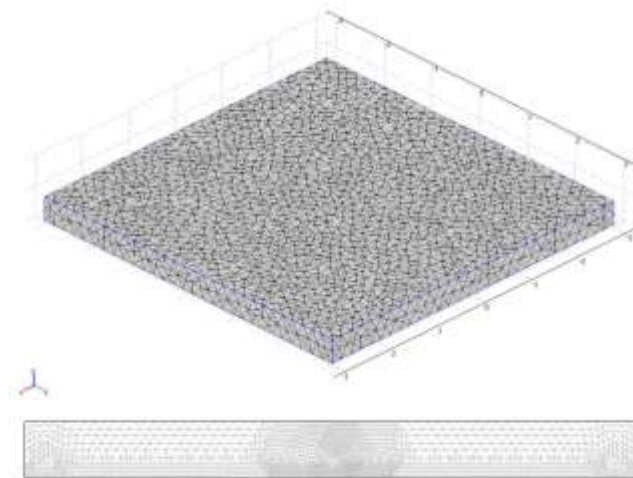
Fig. 2 Total 3D and 2D (section) mesh visualization
