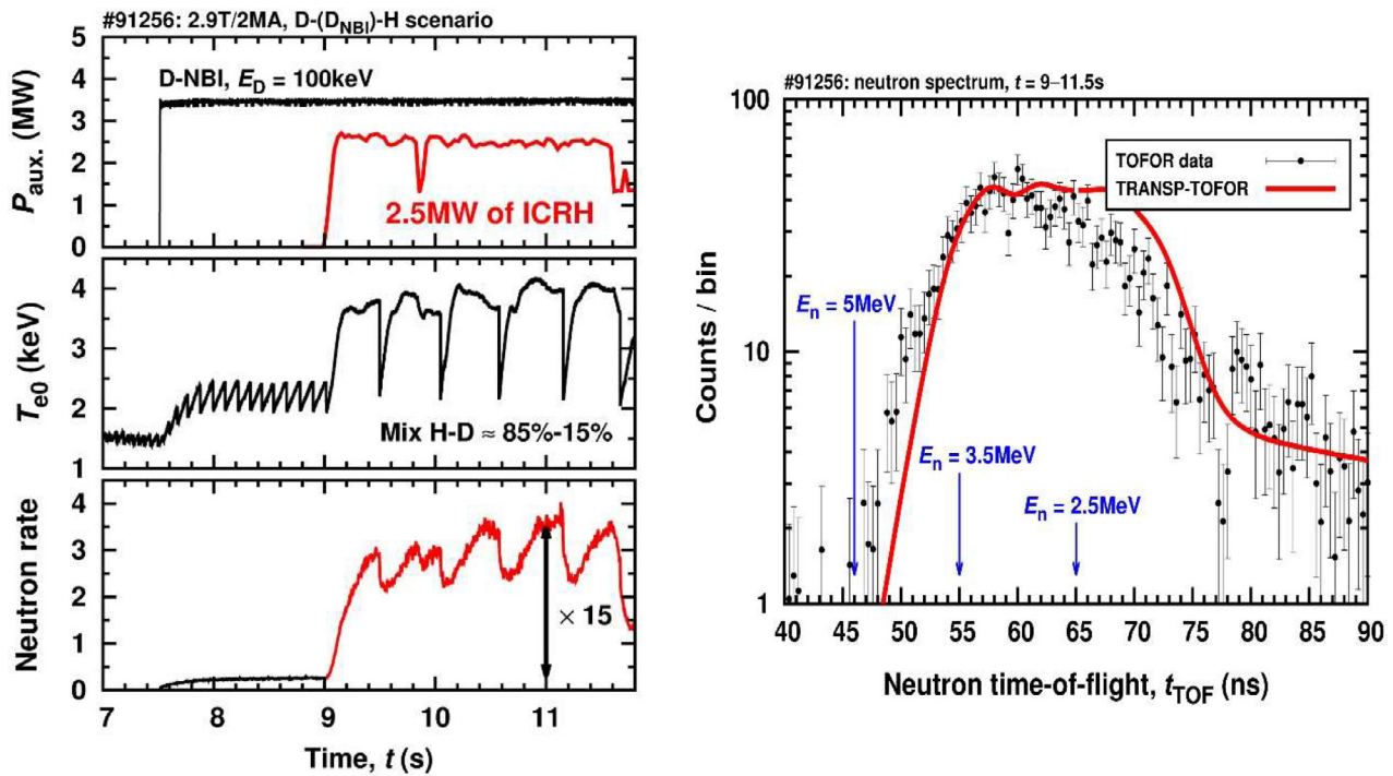
Figure 7. (a) Performance of the three-ion scheme D-(DNBI)-H scenario on JET-ILW (for H/D \sim 6 , n_{e0} = 4 \times 10^{19} \text{ m}^{-3} , f_{ICRH} = 25 MHz, dipole phasing). Note the sharp increase of neutrons during the ICRH pulse. (b) For the pulse of figure 6(a), comparison of the TRANSP synthetic neutron spectroscopy time-of-flight diagnostics with the actual data of the diagnostics showing good agreement between the two. Reproduced courtesy of IAEA. Figure from [67]. Copyright 2018 IAEA.
