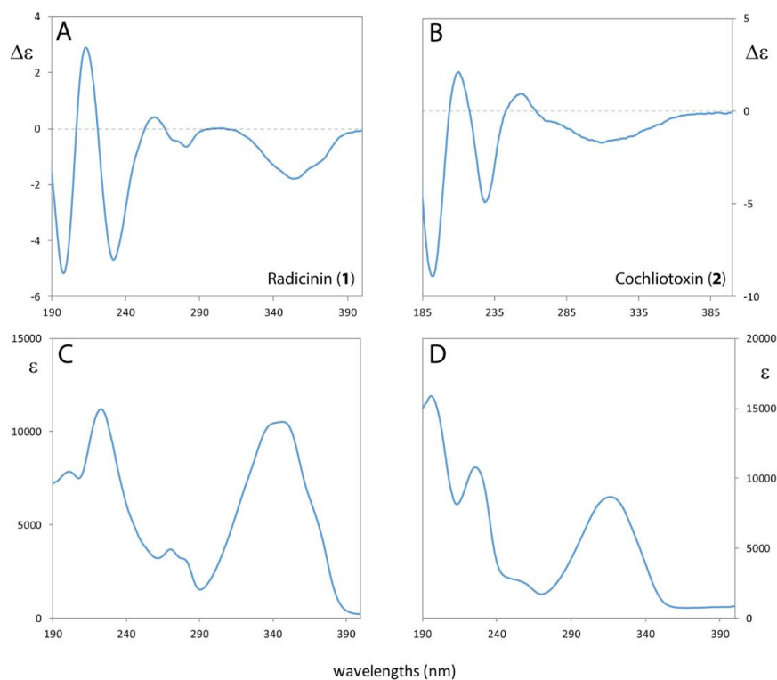
Figure 3. Experimental ECD and UV spectra of radicinin ( 1 ) (panels A,C ) and of cochliotoxin ( 2 ) (panels B,D ) in acetonitrile solution.
