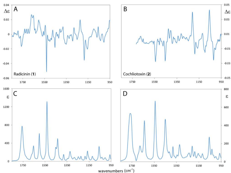
Figure 2. Experimental Vibrational Circular Dichroism (VCD) and IR spectra of radicinin ( 1 ) (panels A,C ) respectively and of cochliotoxin ( 2 ) (panels B,D ) in \text{CDCl}_3 solution. (See Figure S1 of Supplementary Material for the VCD noise level).
