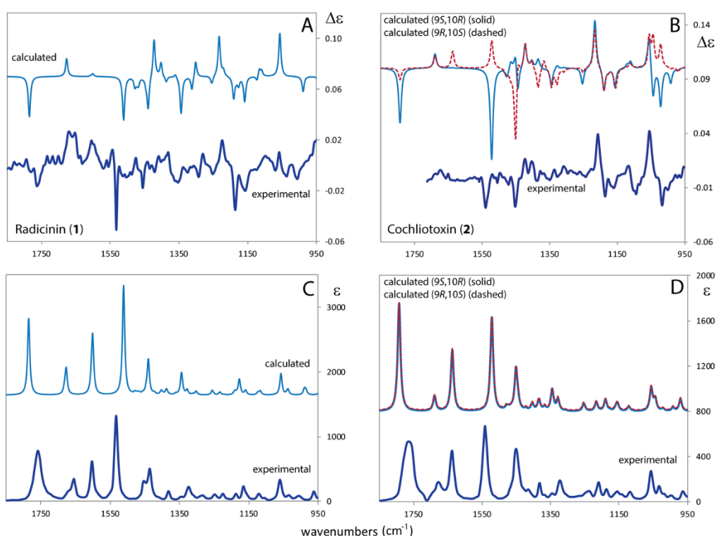
Figure 4. Comparison of experimental and calculated VCD and IR spectra of radicinin ( 1 ) (panels A,C) and of cochliotoxin ( 2 ) (panels B,D). For ( 2 ) the two possible diastereomers have been calculated. DFT/B3LYP/TZVP/PCM( \text{CHCl}_3 ) level of theory. Applied scaling factor is 0.99. Calculated IR spectra are divided by factor of 3.
