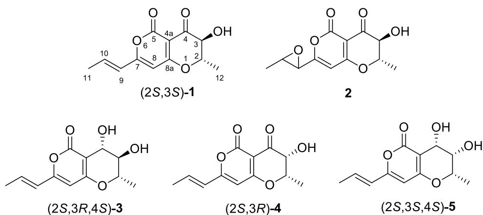
Figure 1. Structure and assigned absolute configuration of radicienin ( 1 ) and of its structural analogue cochliotoxin ( 2 ) and of radicol ( 3 ), 3- epi -radicienin ( 4 ), and 3- epi -radicol ( 5 ). Compounds 1 and 2 are treated in the text, while the chiroptical data of compounds 3–5 are treated in the Supplementary Material.
