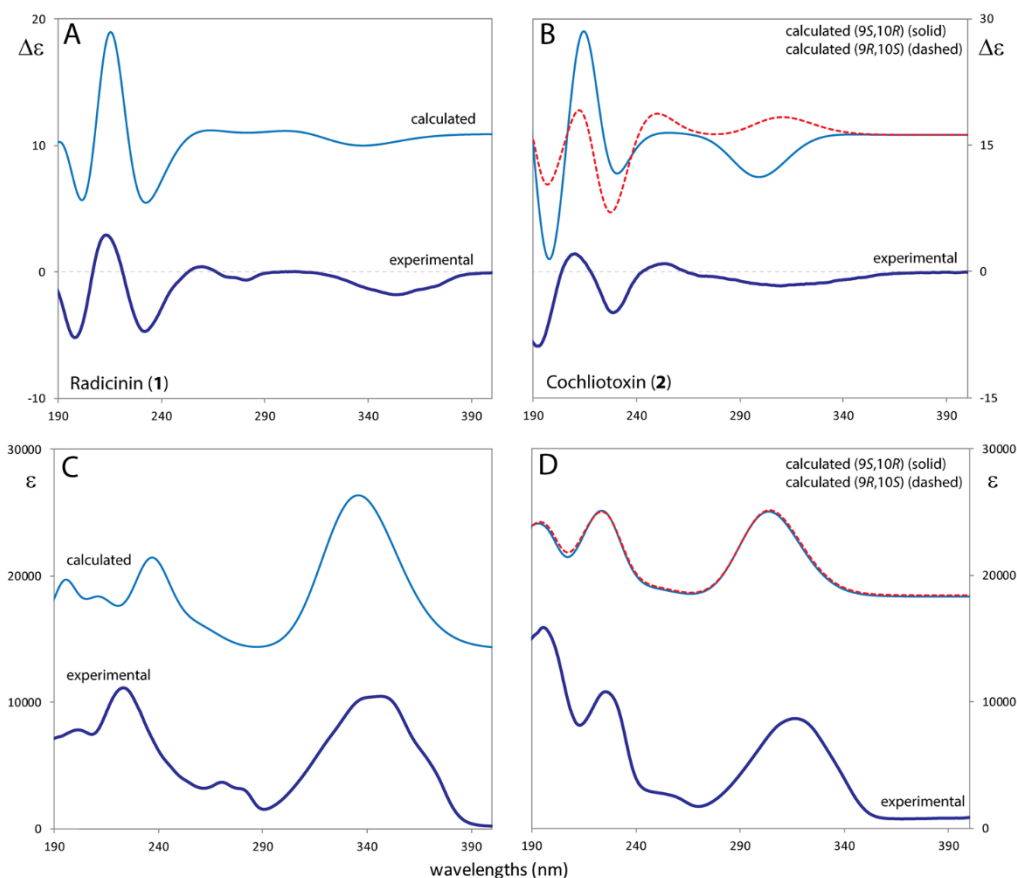
Figure 5. Comparison of experimental and calculated Electronic Circular Dichroism (ECD) and UV spectra of radicinin ( 1 ) (panels A,C) and of cochliotoxin ( 2 ) (panels B,D). For ( 2 ) the two possible diastereomers have been calculated. TD-DFT/CAM-B3LYP/aug-cc-pVDZ/PCM(ACN) level of theory. Calculated spectra are red-shifted by 15 nm and divided by factor 3.
