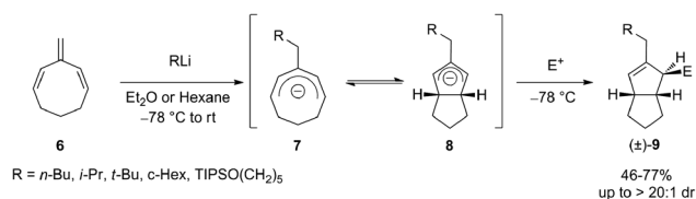
Scheme 4 Carbolithiation of cyclic triene 6.
