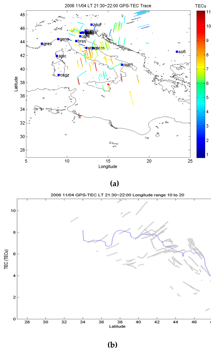
Figure 8. (a) Locations of 17 ground-based Global Positioning System (GPS) receivers (SOPAC, http://sopac.ucsd.edu/ ) and their GPS total electron content (TEC) ground traces during 9:30–10:00 p.m. on 4 November 2006. Blue squares and color curves in the top panel stand for the ground-based GPS receivers and the TEC at its associated ionospheric point, respectively. (b) GPS TEC variations along the volcano longitude during 9:30–10:00 p.m. LT on 4 November 2006. Grey and blue curves in the bottom panel denote the GPS TEC in the network and their median within 10–20 longitude (with a 0.1-deg latitudinal grid), respectively.
