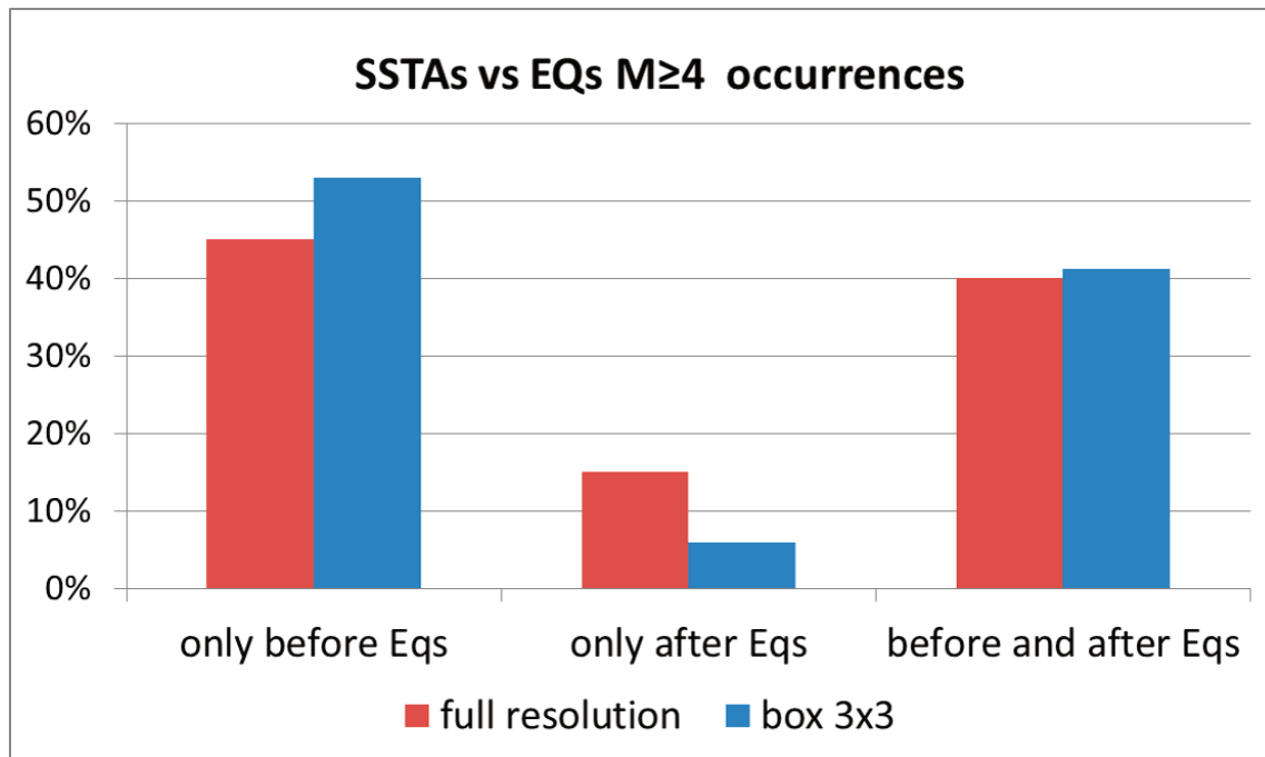
Figure 3. Distribution of the SSTAs compared to earthquake occurrences. For both analysis, more than the 80% of SSTAs associable to earthquakes has tendency to anticipate the occurrence of earthquakes.
