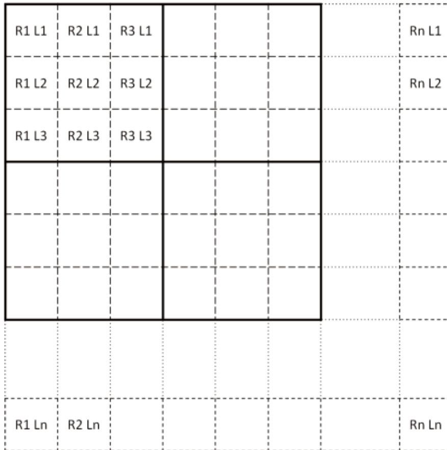
Figure 1. Schematic representation of the applied spatial filter. Dashed lines represent the original full resolution SEVIRI pixels; instead, continuous lines the downscaled resolution SEVIRI pixels. Every three pixels the spatial mean value has been computed only if 5 out of 9 pixels within a region of 3 \times 3 pixels centered on the considered pixel were not affected by clouds.
