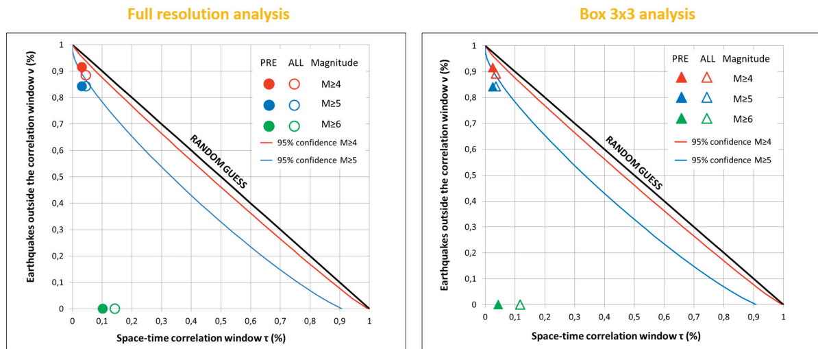
Figure 5. On the left side, Molchan error diagram analysis computed for different classes of magnitude and SSTA identified by applying the RST approach on SEVIRI TIR images at full resolution on the whole study period (2004–2014), while on the right side the corresponding Molchan error diagram computed to SSTA identified by applying the RST approach on SEVIRI TIR images at downscaled resolution. Full circles and full triangles refer to earthquakes occurred only after the appearances of SSTAs (pre-seismic anomalies). Empty circles and empty triangles refer to earthquakes occurred before or after the appearances of SSTAs (earthquake-related anomalies). Red line and blue line indicate the 95% confidence limit curves surrounding the diagonal of random guess for earthquakes with magnitudes greater than 4 and 5, respectively.
