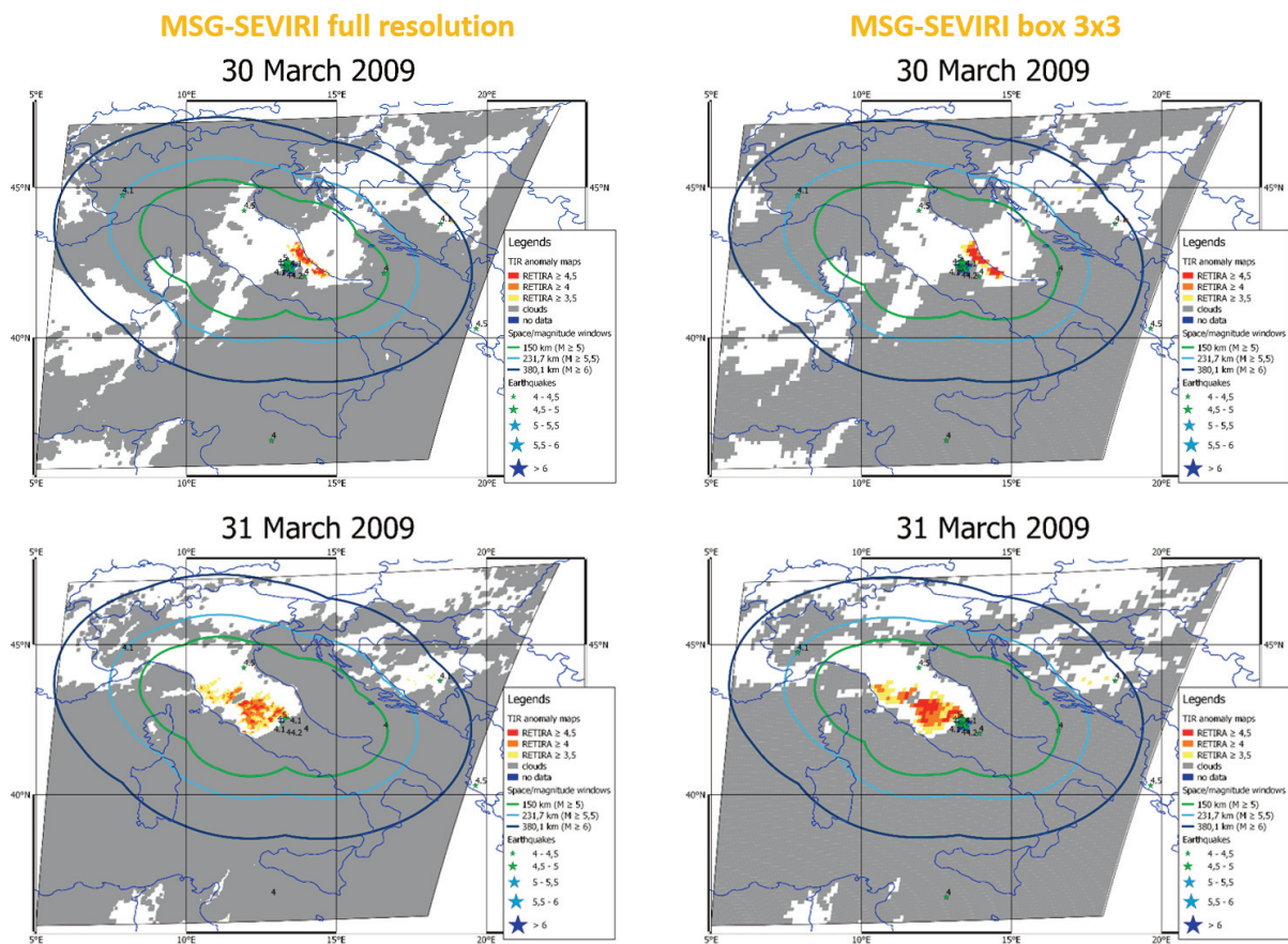
Figure 2. Comparison between Thermal Anomalies Maps (TAMs) obtained by the two RST analyses. On the left side, a Significant Sequence of Thermal Anomalies (SSTA) identified by applying the RST approach on SEVIRI TIR images at full resolution, while on the right side the corresponding SSTA identified by apply the RST approach on SEVIRI TIR images at the downsampled resolution. In both cases, TIR anomalies ( S/N \geq 3.5 ) are depicted in different colors according to the RETIRA (or RETIRA_{\text{box}} ) index values and clouds are depicted in gray. Contours in different colors correspond to different space/magnitude windows (see text) and stars correspond to earthquakes. Significant TIR anomalies (i.e. not due to spurious effects, with spatial extension and temporal continuity) appear in the central part of Italy on March 30 and March 31, 2009, respectively 7 and 6 days before LAquila earthquake ( MW \sim 6.3 ) happened on April 6, 2009.
