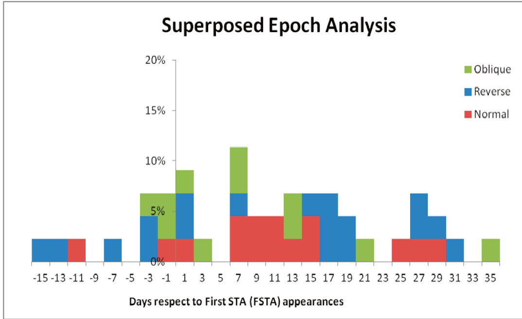
Figure 4. Superposed Epoch Analysis (SEA) between the SSTAs identified by the RST analysis and the RETIRA box index and the seismic events occurred in the investigated region and period. Results have been differentiated on the basis of earthquake focal mechanisms (red indicates earthquakes due to normal faulting, blue earthquakes due to reverse faulting and green earthquakes due to not predominant faulting type, i.e. oblique).
