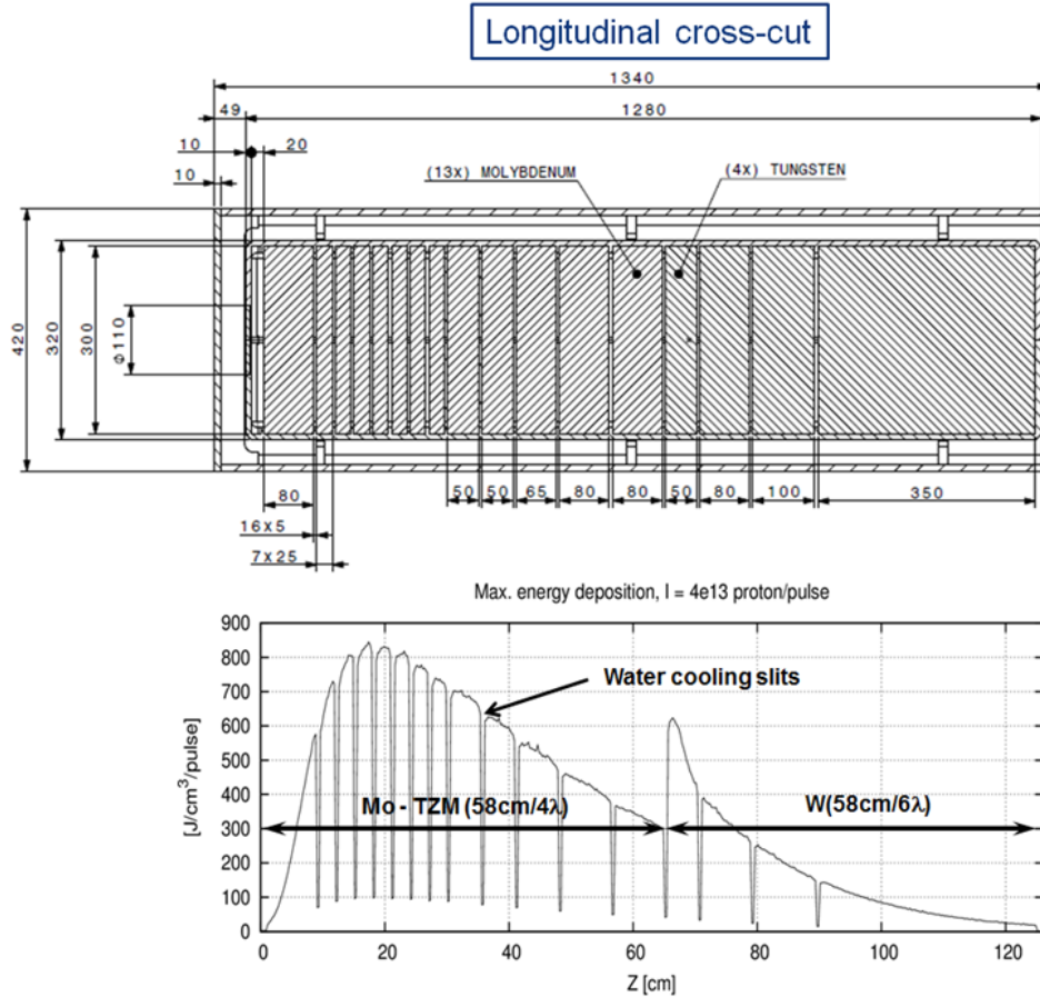
Figure 10. (Top) Preliminary design of the proton target configuration. All dimensions are in mm. The right-slanted hatched region in the top drawing shows the TZM blocks and the left-slanted hatched region the tungsten blocks. (Bottom) Peak energy deposition in the proton target during a spill of 4 \cdot 10^{13} protons.
