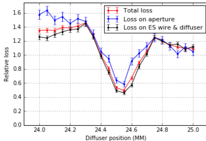
Figure 7. Relative loss of protons in arbitrary units as a function of the transverse position from simulation of a 3 mm long, 0.24 mm wide tungsten-rhenium diffuser. The sum of the loss on the diffuser and the electro-static septum (ES) wires is lower than the total loss with ES wires alone, because the scattering from the diffuser reduces the particle density at the ES sufficiently to result in an overall loss reduction. A factor two improvement is obtained for the optimal position.
