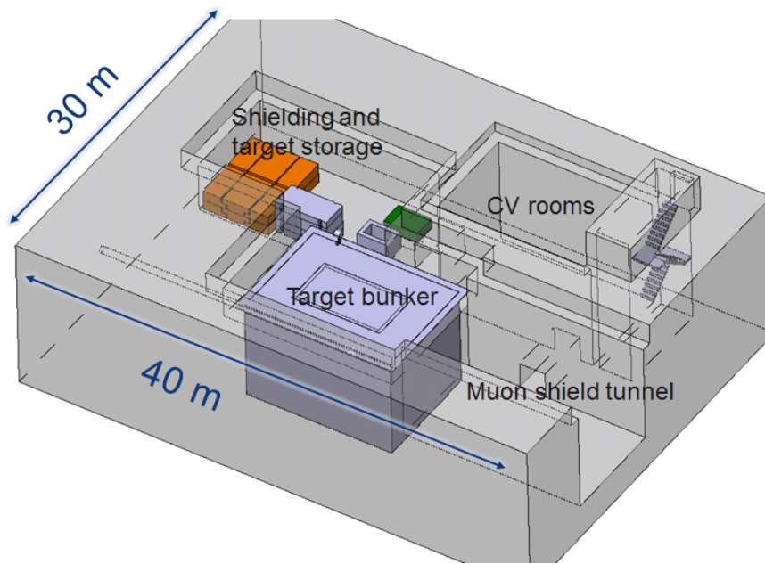
Figure 11. Overview of the main components of the target complex. The proton beam line arrives from the left of the target bunker. The target is located in the centre of the target bunker and the first section of the muon shield in terms of the magnetized hadron stopper is integrated in the downstream end of the bunker.
