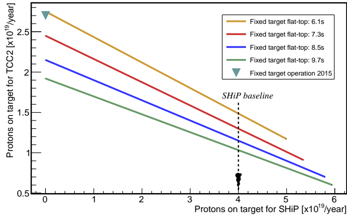
Figure 6. The expected number of protons on the current North Area targets (TCC2) as a function of the number of protons on target for the SHiP experimental facility. The plot shows the performance for different spill durations for the current targets. The expected integrated number of protons for exclusive operation of the North Area targets with the super-cycle used in 2015 is indicated by a triangle. The preferred working point for SHiP is indicated by "SHiP baseline".
