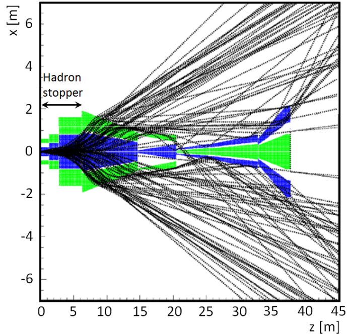
Figure 12. Horizontal cross-section of the muon shield magnet configuration at the level of the beam-axis ([18], reproduced here for completeness). The direction up/down of the vertical magnetic field is illustrated by the blue/green colour of the iron poles of the magnets. Typical trajectories of muons across the momentum spectrum are overlaid.
