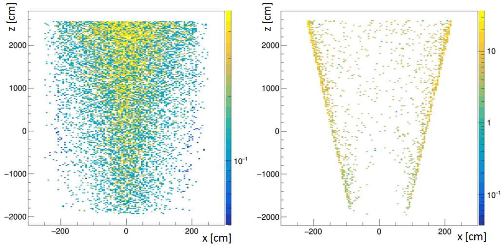
Figure 13. Vertex distribution of signal candidates produced by neutrino interactions from 2 \cdot 10^{20} protons on target assuming air at atmospheric pressure in the fiducial volume with a soft selection for Heavy Neutral Leptons (left), as compared to the situation with a vacuum vessel evacuated down to a pressure of 10^{-3} bar (right).
