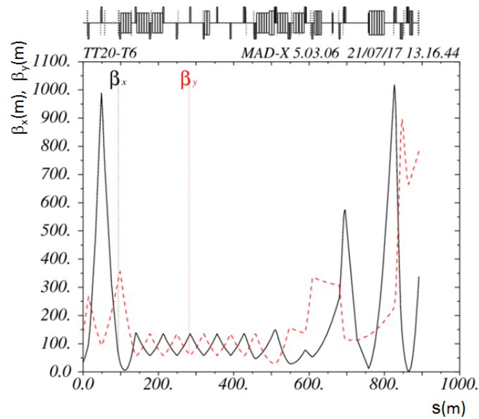
Figure 9. Optics shown by the beta function in the horizontal (black solid line) and vertical plane (red dashed line) along the entire length of the beamline from the SPS extraction ( s = 0 m) in LSS2 to the SHiP proton target located at around s = 900 m. The new section of beamline is matched to the existing TT20 line to give the required beam size at the target.
