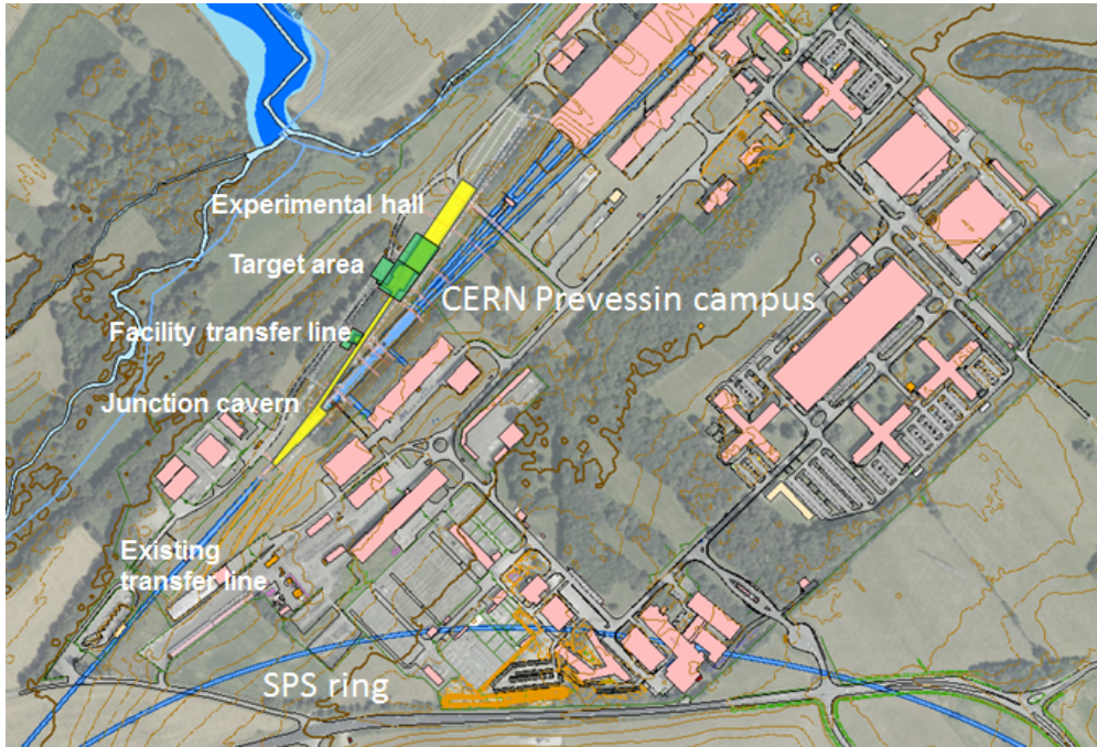
Figure 3. Overview of the required civil engineering for the proposed experimental facility for SHiP on the CERN Preveessin campus. The beam-axis is at a depth of about 10 m which allows trenching the entire complex from the surface. New or reworked construction in yellow (underground) and green (surface); existing tunnels in blue.
