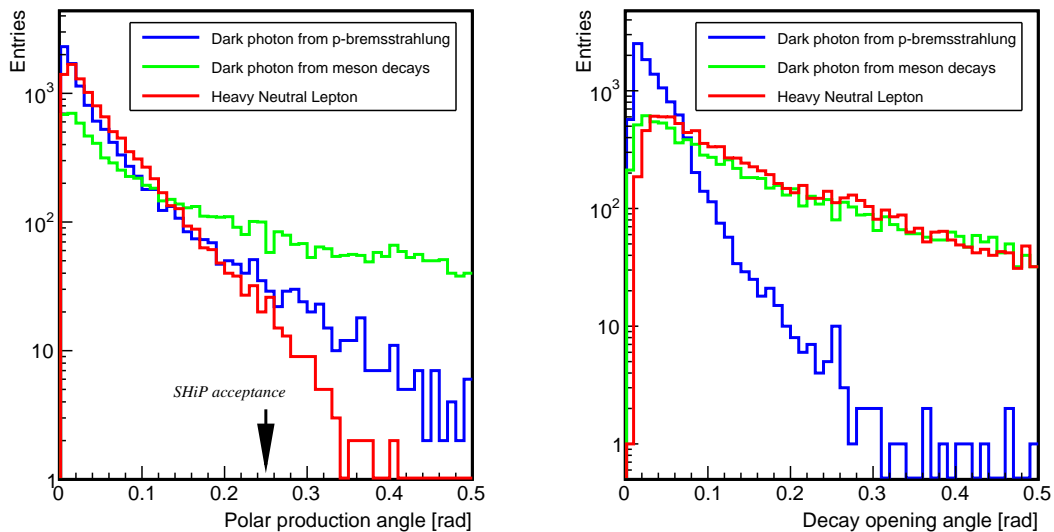
Figure 1. (Left) Polar production angle with a beam momentum of 400 \text{ GeV}/c for Dark Photons ( A ) produced in proton bremsstrahlung ( m_A = 2.0 \text{ GeV}/c^2 ) and in meson decays ( m_A = 0.9 \text{ GeV}/c^2 ), and for Heavy Neutral Leptons (HNL) ( m_{HNL} = 1.0 \text{ GeV}/c^2 ) from decays of charm hadrons. (Right) Decay opening angles for two-body decays of the same three cases.
