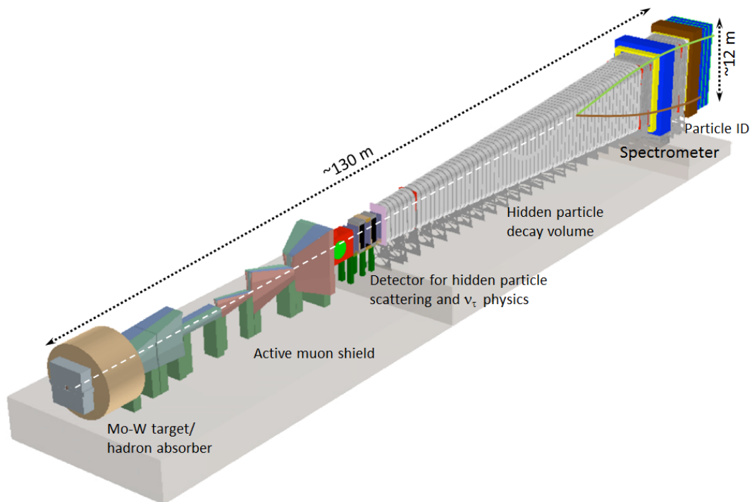
Figure 2. Overview of the target and experimental area for the SHiP detector as implemented in the physics simulation.
