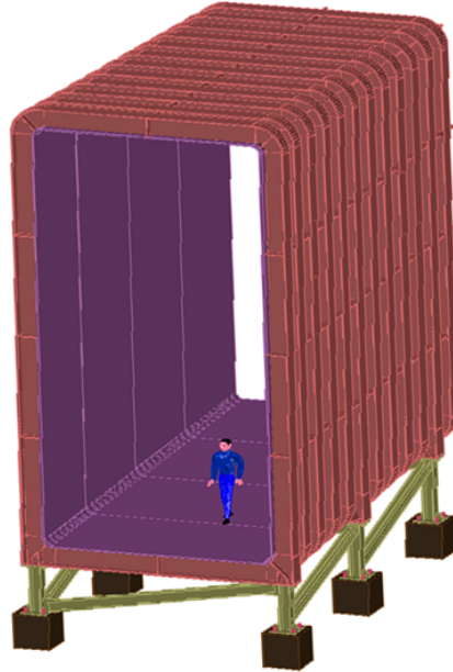
Figure 14. Cross-sectional view of the vacuum vessel which provides a pressure of O(10^{-3}) bar in the decay volume. The design has been optimized in order for the wall to be as light and as slim as possible, and to incorporate a detector system which tags background events.
