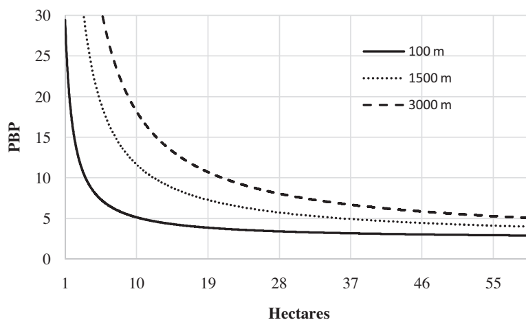
Fig. 5. Payback period calculated for an SRF plantation sited at distances of 100 m, 1500 m, 3000 m.
