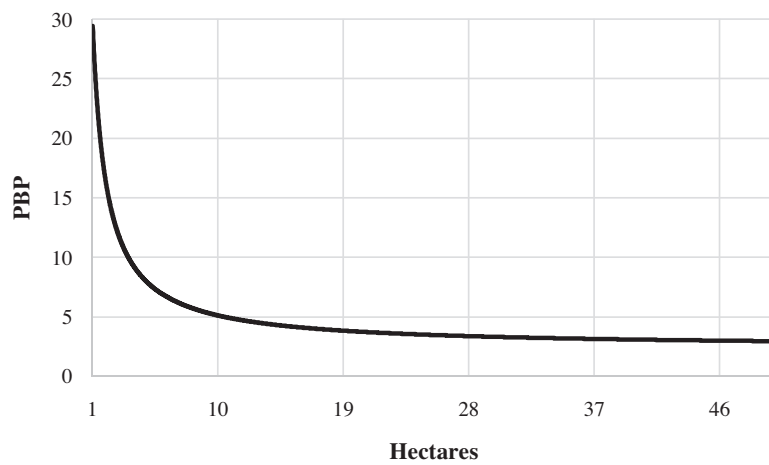
Fig. 4. Payback period for a SRF plantation sited at 100 m from the WWTP.
