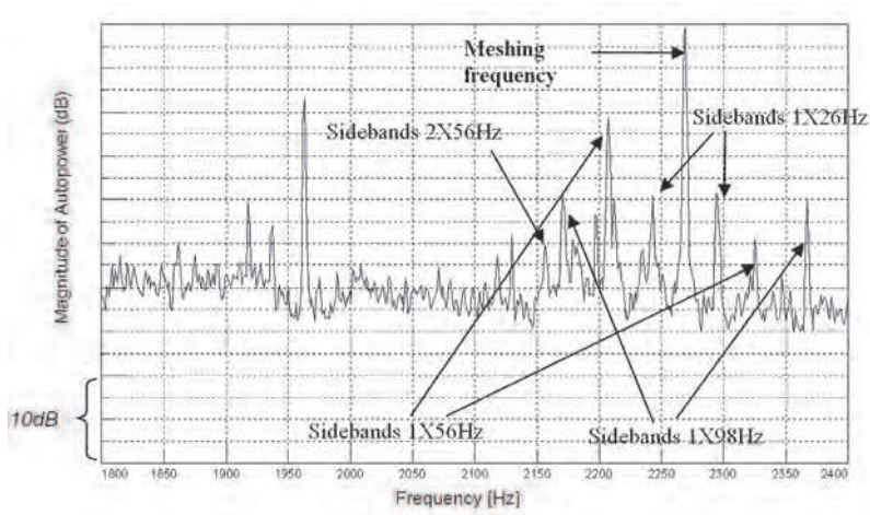
Fig. 11. Autopower of acoustical pressure. Zoom of Figure 10 around a meshing frequency (from 1800Hz to 2400Hz). Meshing frequency and relative sidebands spaced at 26Hz, 56Hz, and 98Hz.
