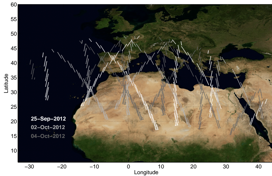
Figure 7. Footprint positions of IASI observations for the GSICS IASI/SEVIRI Inter-calibration experiment.
