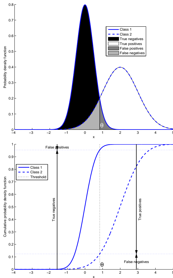
Figure 4. Visual representation of Type I and II errors by density (top panel) and cumulative (bottom panel) probability functions.
