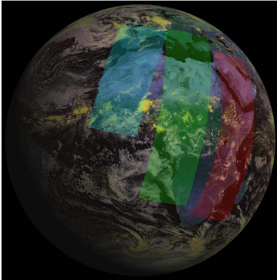
Figure 6. SEVIRI full disk imagery starting at 09:27:43 UTC for the day 22 July 2007. The target area used to check the cloud detection scheme is that encircled within red lines.
