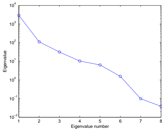
Figure 5. Example of covariance matrix of the vector x for the case of the tropical climate zone and sea surface; top panel, covariance matrix; bottom panel, eigenvalues.
