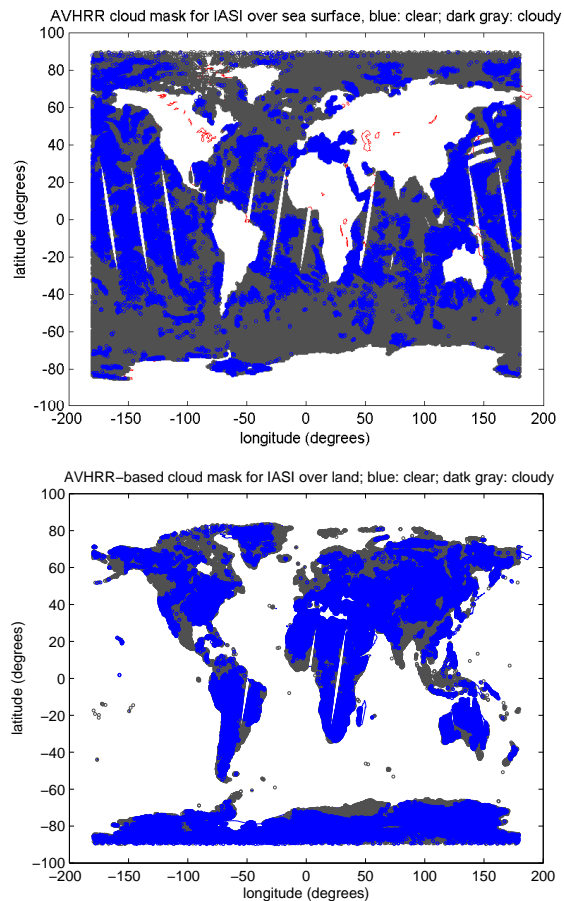
Figure 1. IASI cloud mask derived from AVHRR for the set IASI2; top panel: sea surface; bottom panel: land surface. Blue color refers to clear sky and dark gray to cloudy one.
