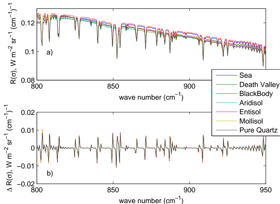
Figure 3. Top panel: radiance spectra in the atmospheric window segment [800\text{--}950] \text{ cm}^{-1} for very different surface emissivities. Bottom panel: the same radiance spectra after first order differentiation. The synthetic spectra have been obtained with the same state vector, but emissivity.
