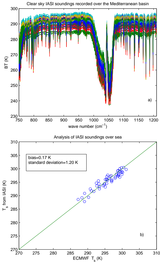
Figure 2. Example of the performance of the split window technique for the estimation of the skin temperature. (b) compares the IASI T_s obtained from the spectra shown in (a) with the time-space co-located ECMWF analysis.
