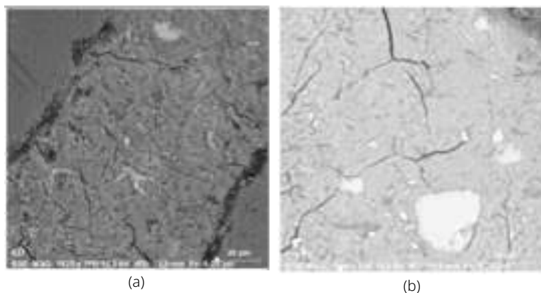
Figure 2. SEM micrographs illustrating the influence of nano-silica on mortar microstructure. (a) Reference mortar showing typical capillary pore structure. (b) Mortar containing an intermediate nano-silica dosage showing matrix densification and refined pore distribution.
