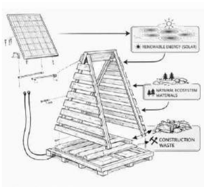
Figure 4. Exploded axonometric view of the same device, illustrating the origin of the materials used in relation to the Local Atlas of Energy and Matter.
