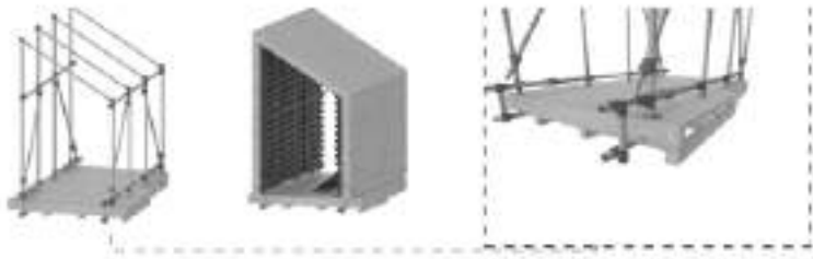
Figure 4. Details of the constructive joints and ballast foundation platforms. [Source: see Note 1].
