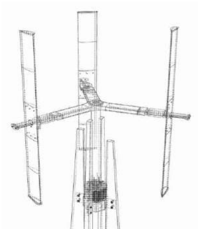
Figure 5. Micro-VAWT blades' technical drawing: detail. [Source: authors, courtesy of Ivan Del Ponte].
