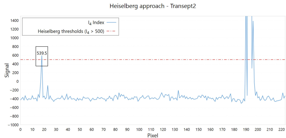
Figure 13. The plot shows the spatial distribution of the I_4 index proposed by Heiselberg P. and Heiselberg H. [40] along “Transept2”; the black-bordered square indicates the pixel (no. 18) where a false positive occurs.
