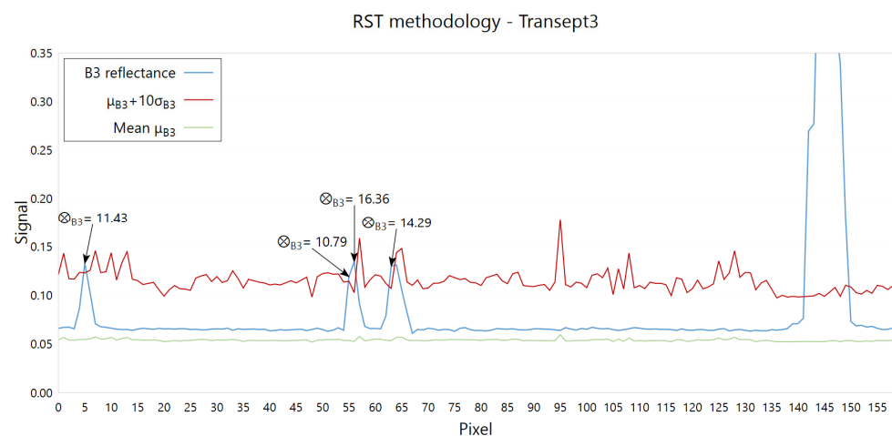
Figure 17. Spatial distribution along “Transept3” of reflectance values in the VIS band (B3 of S2) and related parameters used by the RST-based iceberg detection. The arrows highlight the pixels (with \otimes_{B3} > 10 ) identified as “candidate icebergs,” also reporting the associated \otimes_{B3} value.
