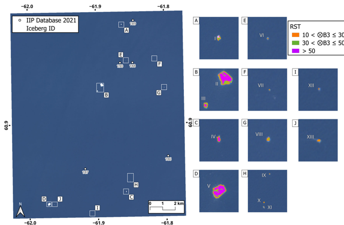
Figure 10. Application of the RST approach to the S2 image of 10 August 2021 at 15:39 (UTC) within the Labrador Sea (RGB in background). The spatial distributions of \otimes_{B3} values around the icebergs identified at \otimes_{B3} > 10 are displayed in the insets on the right (A–J), together with their RST identifier numbers (I to XIII).
