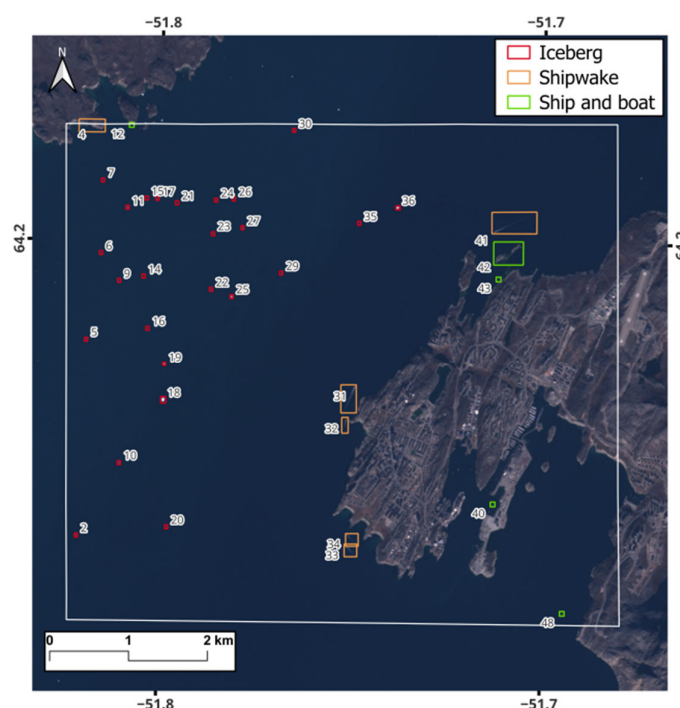
Figure 1. Results by Heiselberg P. and Heiselberg H. [40] over Nuuk (Greenland) based on the S2 (Level 2A) image (tile 22 WDS) collected on 26 September 2016 (RGB in background). Different
