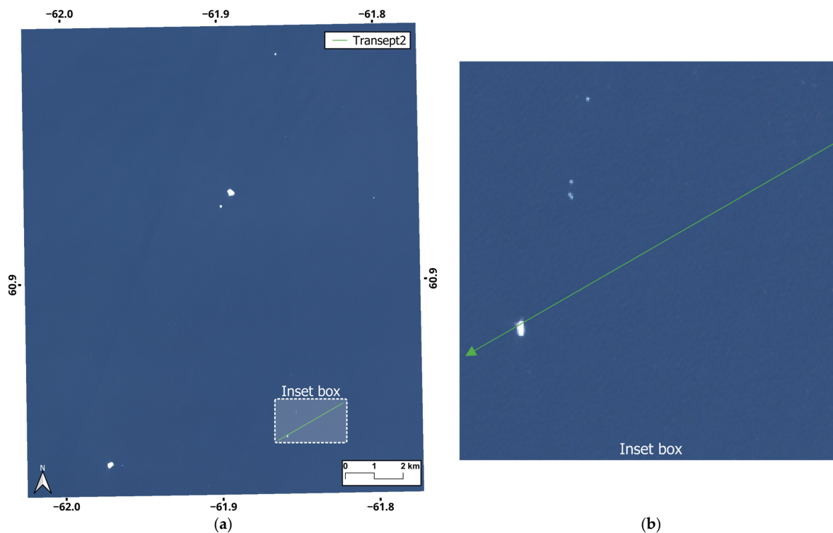
Figure 12. MSI-S2 image acquired in the Labrador Sea AOI on 10 August 2021 (RGB in background): (a) geographical location of “Transept 2” (dashed white box) and (b) close-up view of the green transect that intersects the iceberg (IIP n. 186, RST id n. IV).
