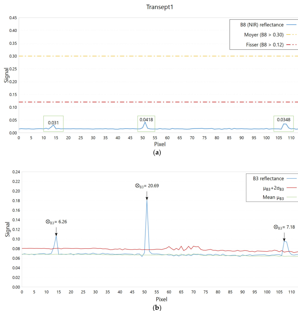
Figure 9. The graphs show the signal trend along transept 1; (a) shows the spatial distribution of reflectance in band 8 (NIR) along “Transept1” within the image acquired by S2, as well as the corresponding thresholds proposed by Moyer [41] and Fisser [46]. Green-bordered squares indicate
