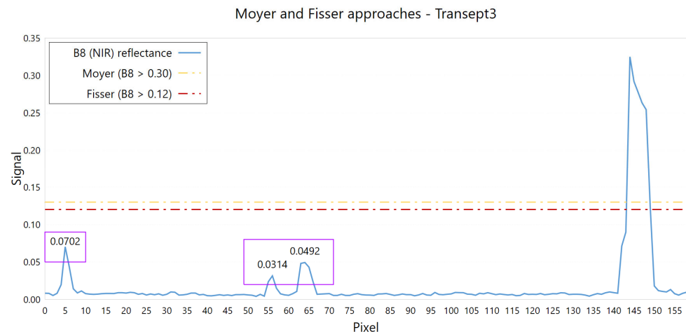
Figure 16. Spatial distribution along “Transept3” of reflectance values in the NIR band (B8 of S2) and the corresponding thresholds set by Moyer [41] and Fisser [46] for iceberg detection. The purple boxes highlight the pixels corresponding to the three “candidate icebergs” not identified by the two fixed threshold methods.
