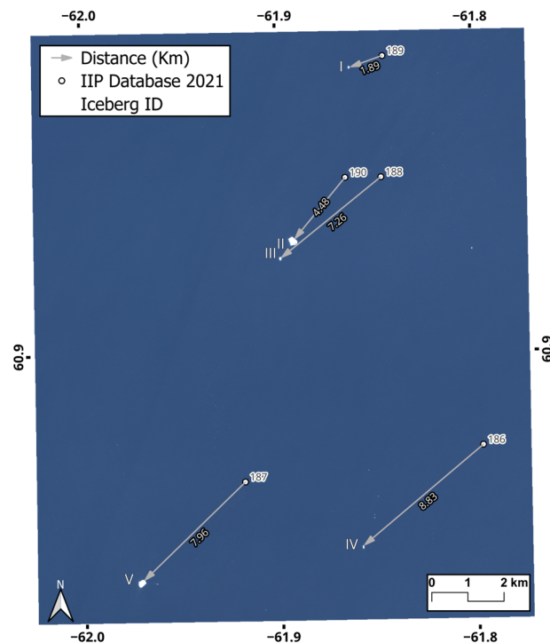
Figure 11. Distance between the positions of the five icebergs recorded in the IIP database, sighted at 08:52 UTC on 10 August 2021 in the Labrador Sea AOI, and the ones (numbered from I to V) detected by RST within the image acquired by S2 on the same day at 15:39 UTC (RGB background).
