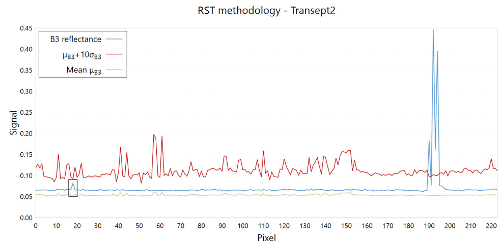
Figure 14. The graph highlights the spatial distribution, along the “Transept2” of the parameters used in the RST methodology to identify anomalous values associated with icebergs. The black-bordered square indicates the pixel no. 18 with no associated anomalies. Note that the large iceberg reported as n. 186 by the IIP is correctly identified by RST (as n. IV) at pixels 190, 192–194, with \otimes_{B3} values well above 10 (from 20 up to 70).
