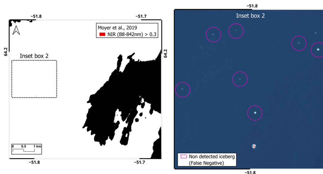
Figure 3. Results of the application of the fixed-threshold algorithm for iceberg detection using NIR band proposed by Moyer et al. [41]. The inset box 2 shows the position of some of the undetected icebergs in the area of interest, circled in bright pink (RGB background). Image Level 1C was acquired on 26 September 2016 by the Sentinel-2 constellation, tile 22 WDS.
