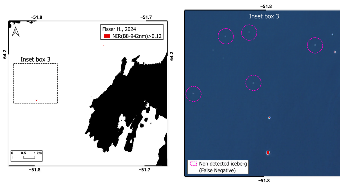
Figure 4. Results of the application of the fixed-threshold algorithm proposed by Fisser [46] for iceberg detection using the NIR band of the S2 image (Level 1C, tile 22 WDS) acquired on 26 September 2016. The inset box enlarged on the right shows, circled in bright pink, some of the undetected icebergs in the area of interest with RGB background.
