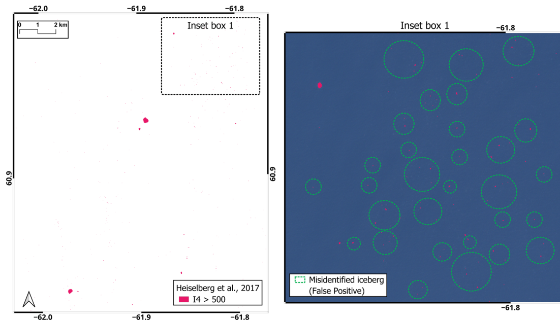
Figure 2. Result of applying the I_4 > 500 index [40] to a portion of the Labrador Sea. Image acquired on 10 August 2021 by S2 (Level 2A), tile 20 VNN. Inset box 1 on the right (RGB in background) shows an area within the region of interest where some of the numerous false positives, highlighted by the green dotted circles, have been detected.
