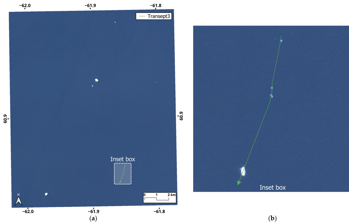
Figure 15. MSI-S2 image acquired in the Labrador Sea AOI on 10 August 2021 (RGB in background): (a) geographical location of “Transept3” (dashed white box) and (b) a detailed view of the area of the dashed white box depicted on the left: the green line (“Transept3”) intersects four icebergs in the area.
