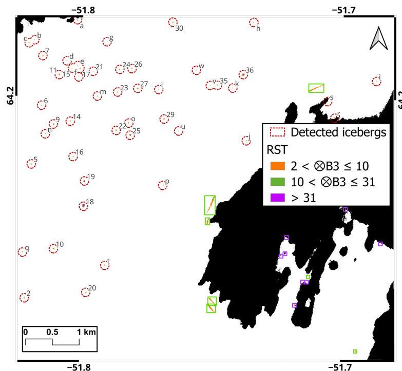
Figure 7. Application of \otimes_{B3} index on the 26 September 2016 at 15:09 (UTC) S2 image in the Nuuk AOI; the result shows \otimes_{B3} > 2 based on three different colour patterns; the mainland is shown in black, using the land–sea mask. The red dotted circles indicate the identified icebergs (labelled with numbers and letters), the green rectangles indicate the boats, and the purple ones highlight the “other objects”.
