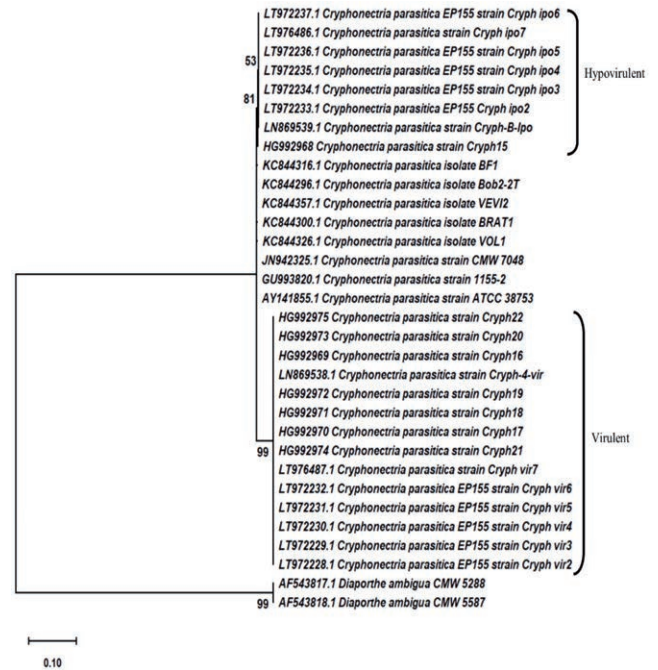
Figure 2. Maximum-Likelihood phylogenetic tree based on ITS gene region (606 bp) of 30 Cryphonectria parasitica isolates. Two ITS nucleotide sequences of Diaporthe ambigua isolates were used as outgroups. The percentage in which the associated taxa clustered together in the bootstrap test (1,000 replicates) is shown below the nodes. Values less than 50% are not revealed. Scale=number of substitutions/site.
