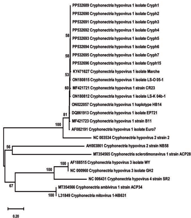
Figure 3. Maximum-Likelihood phylogenetic tree of 24 Cryphonectria parasitica isolates based on polyprotein of ORF B gene (950 bp) of the CHV-1. The percentage in which the associated taxa clustered together in the bootstrap test (1,000 replicates) is shown below the nodes. Values less than 50% are not revealed. The tree is drawn to scale, with branch lengths measured in the number of substitutions/site.
