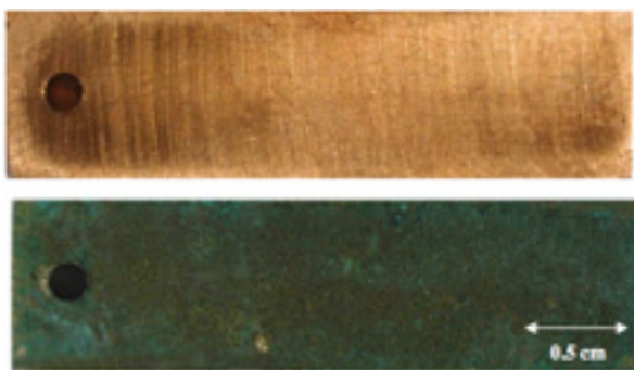
Figure 2. Bronze ingot before and after the corrosion test.
