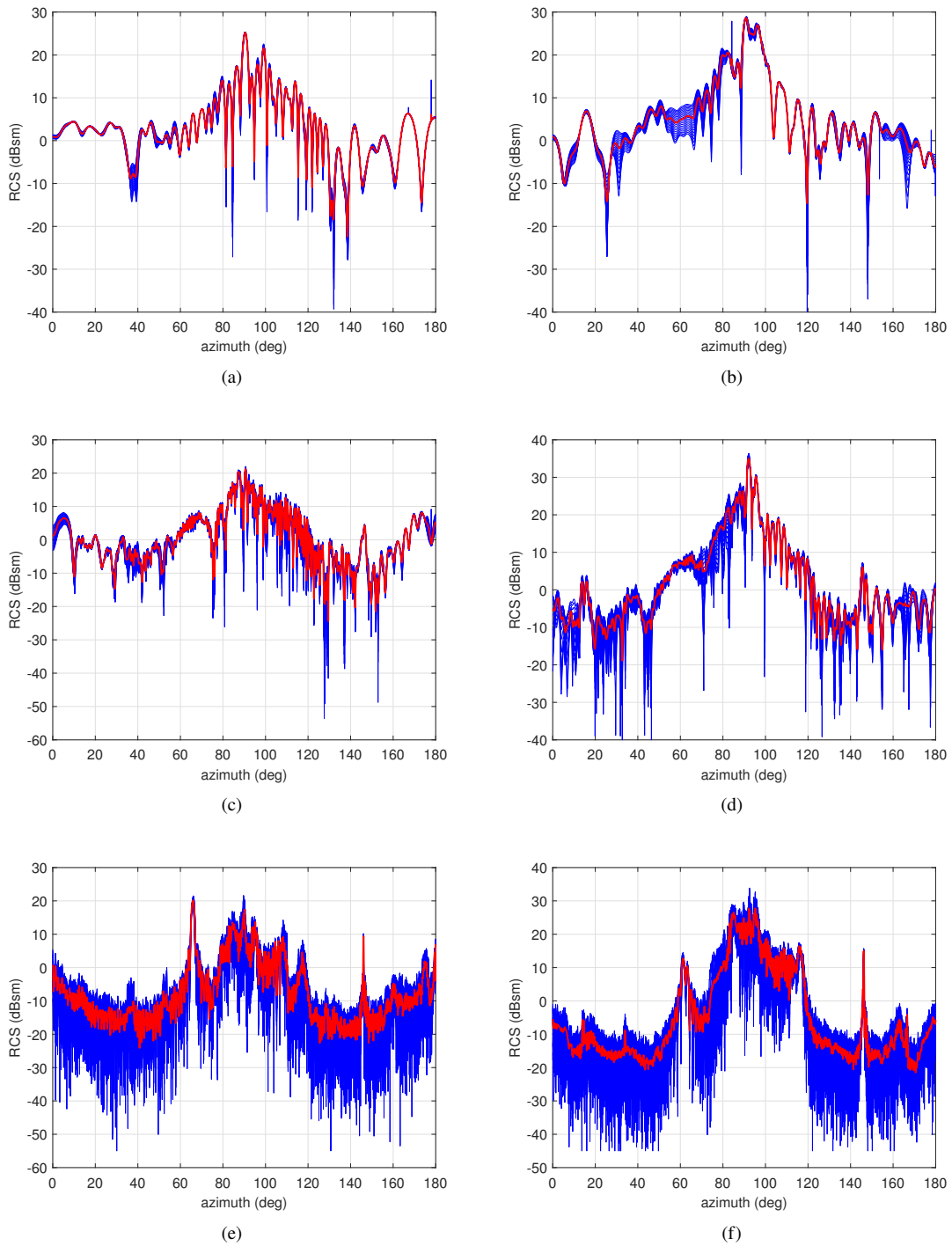
Fig. 2 RCSs (dBsm) (blue line) and its mean value (red line) versus azimuth (in degrees) of the F-35 aircraft, for the three considered frequency band (i.e., VHF, L, and X, from top to bottom) under the LR (left column) and MR (right column) regimes.
