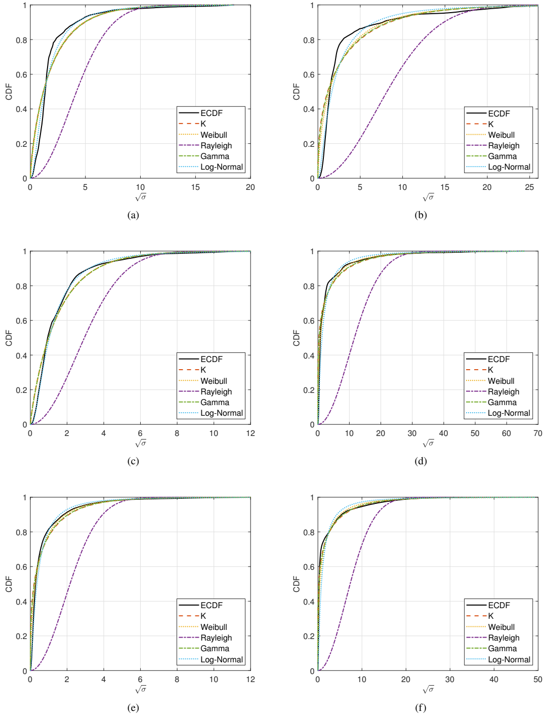
Fig. 3 Theoretical CDF and ECDF versus \sqrt{\sigma} of the F-35 aircraft, for the three considered frequency bands (i.e., VHF, L, and X, from top to bottom) under the LR (left column) and MR (right column) regimes.
