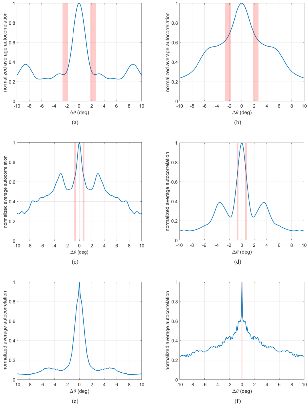
Fig. 4 Normalized average autocorrelation of the RCS of the F-35 aircraft, for the three considered frequency bands (i.e., VHF, L, and X, from top to bottom) under the LR (left column) and MR (right column) regimes.
