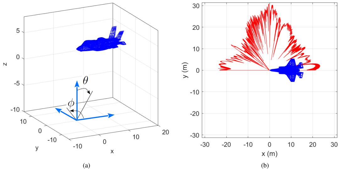
Fig. 1 Reference system (subplot a) and x - y view (subplot b) of the F-35 with overlapped the polar plot of its RCS (dBsm), i.e., for elevation angle varying in the interval [98, 100] deg, and in L-band (operating frequency 1 GHz).
