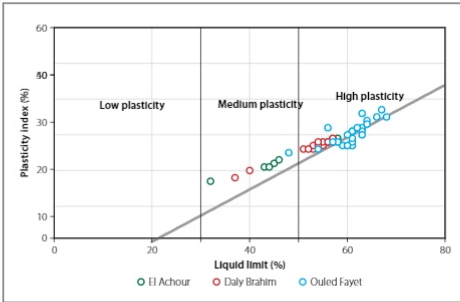
Figure 6 Plasticity chart of the studied soils
