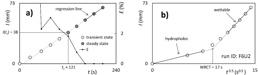
Figure 2. (a) Example of estimation of the equilibration time, t_s (s), and infiltrated depth at the equilibration time, I(t_s) (mm) from cumulative infiltration and (b) water repellency cessation time, WRCT (s), as the intersection point of two straight lines, representing the initial (hydrophobic) and the late (wetttable) stages of the I vs. t^{0.5} plot of a Beerkan infiltration run affected by soil water repellency (SWR).
