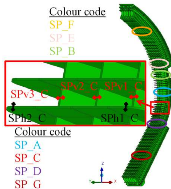
Figure 25. Locations of paths for the stress linearization.
