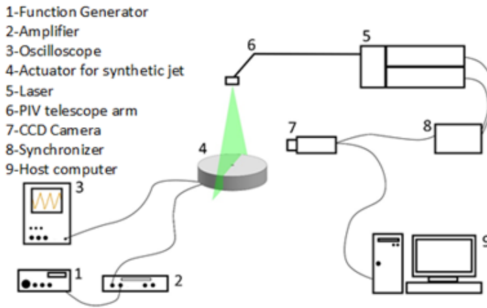
Fig. 8. Schematic representation of the PIV setup adopted
