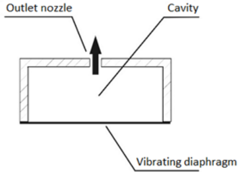
Fig. 1. Schematic representation of a device for synthetic jet generation
