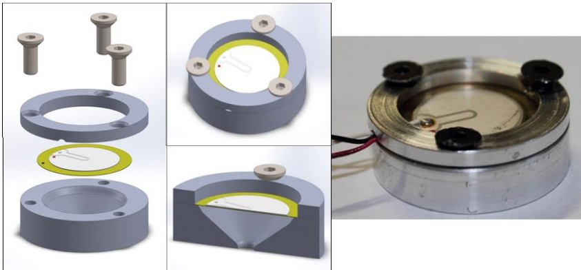
Fig. 3. Device with piezoelectric actuator
