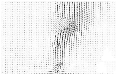
Fig. 15. Velocity distribution of the same jet of the previous figure obtained with a traditional PIV technique
