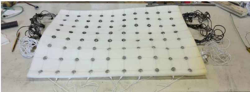
Fig. 6. In this image 80 speakers are uniformly distributed along a blanket 0.35 x 0.45 m
