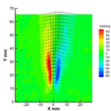
Fig. 12. Average vorticity distribution
