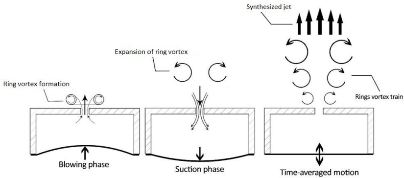
Fig. 2. Qualitative description of the formation of synthetic jet
