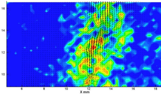
Fig. 16. Overlap of BOS image with a PIV velocity distribution
