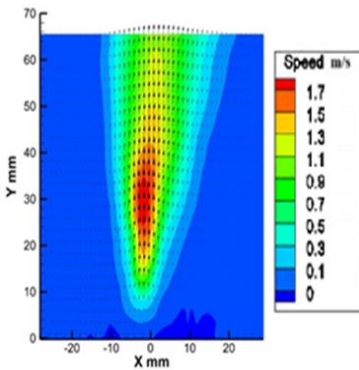
Fig. 11. Average velocity distribution
