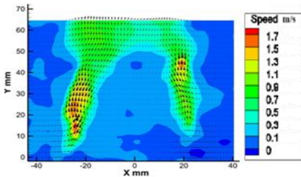
Fig. 13. Instantaneous velocity distribution of two jets
