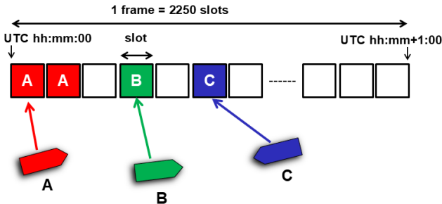
Fig. 1. AIS channel TDMA scheme: each frame is divided into 2250 slots of 26.67 ms, used for AIS message transmissions.
