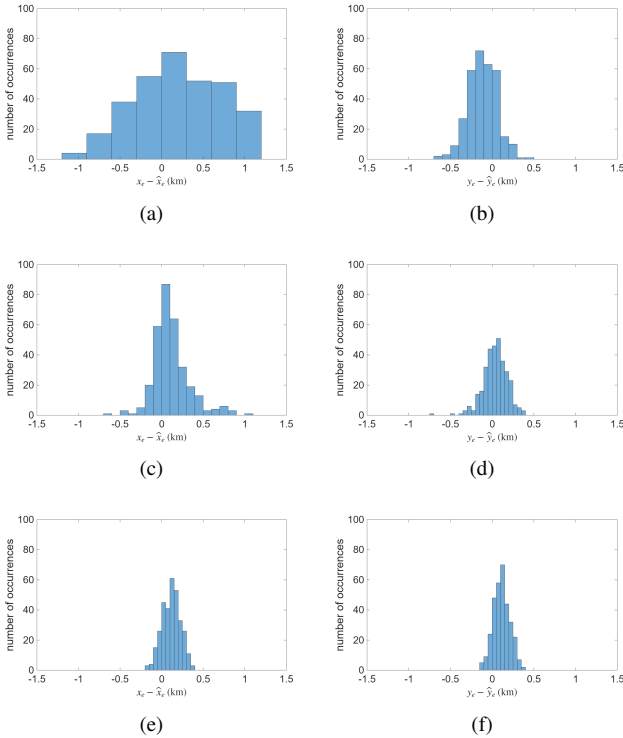
Fig. 5. Histograms of the absolute position estimation errors for the LS-TOA (top line), LS-TDOA (central line), and CLS-TDOA (bottom line) algorithms along the x - (left) and y -axes (right).
