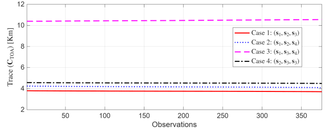
Fig. 7. Trace of the CRB for varying target positions under different sensor configurations.
