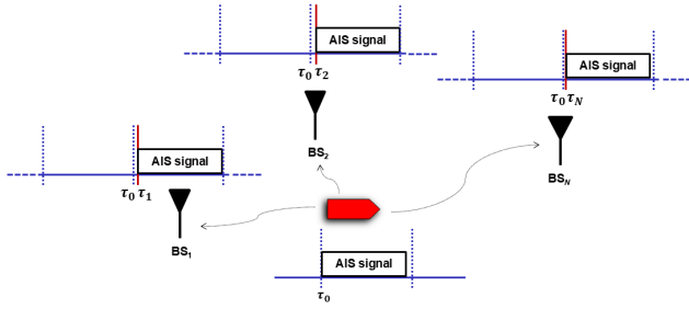
Fig. 2. Pictorial representation of the TOA/TDOA-based passive localization of AIS-equipped vessels using multiple shore-based AIS BSs.
