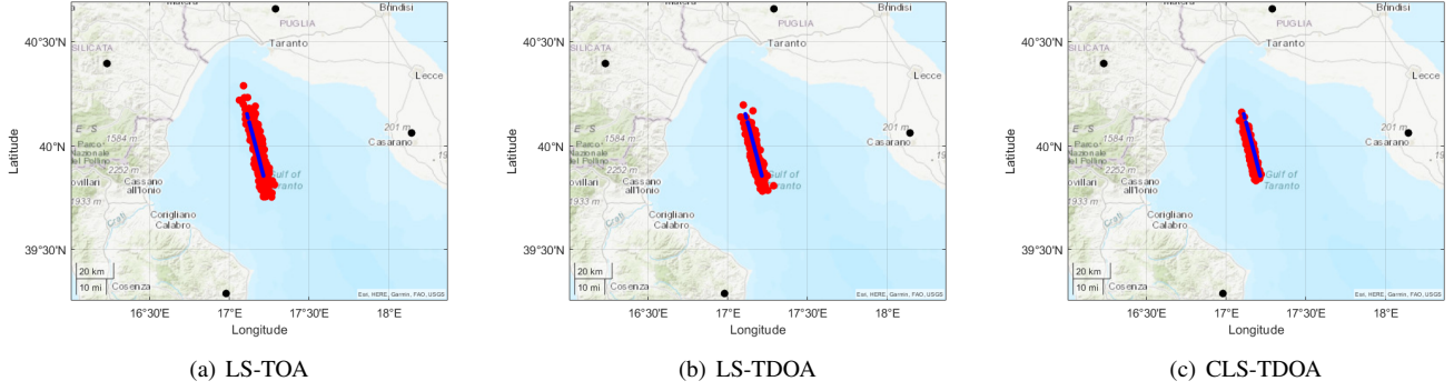
Fig. 4. Results of the LS-TOA, LS-TDOA, and CLS-TDOA positioning algorithms visualized on the topographic map.
