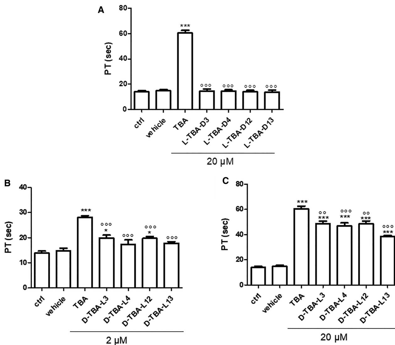
Figure 4. PT values of the enantiomeric TBA derivatives and their natural counterpart at different concentration (2 and 20 \mu\text{M} ) with an incubation time of 15 min. See the main text and the Materials and Methods section for details. * P < 0.05 , *** P < 0.001 versus vehicle, °°° P < 0.001 versus TBA ( n = 3 ).
