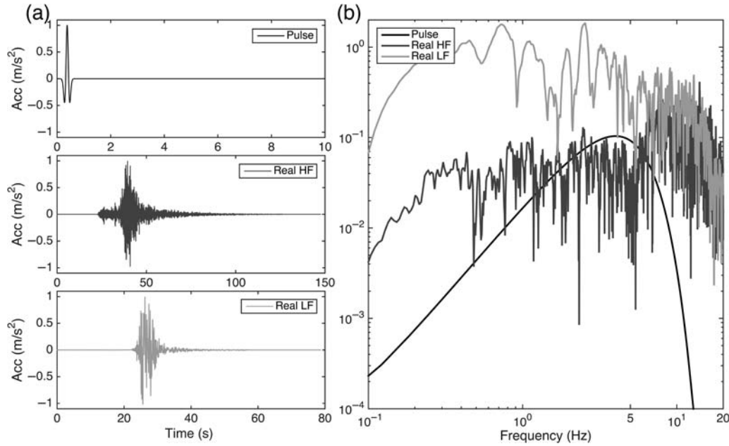
Figure 3. Normalized acceleration of the reference motions used for the verification phase (pulse, real motions: high-frequency [HF] motion and low-frequency [LF] motion) of this PREdiction of NON-LINear soil behavior (PRENOLIN) project (a) with the associated Fourier spectrum (b).
