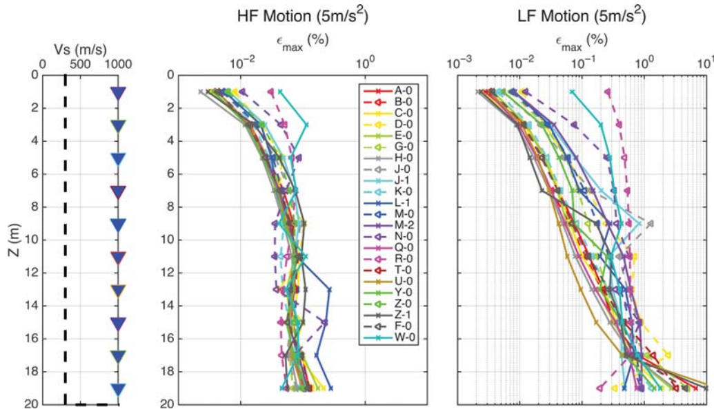
Figure 12. Peak shear-strain profiles reached at each depth by each team for the HF and LF reference motion scaled at the highest PGA level (5 m/s 2 ), for profile 1 and for rigid substratum conditions.
