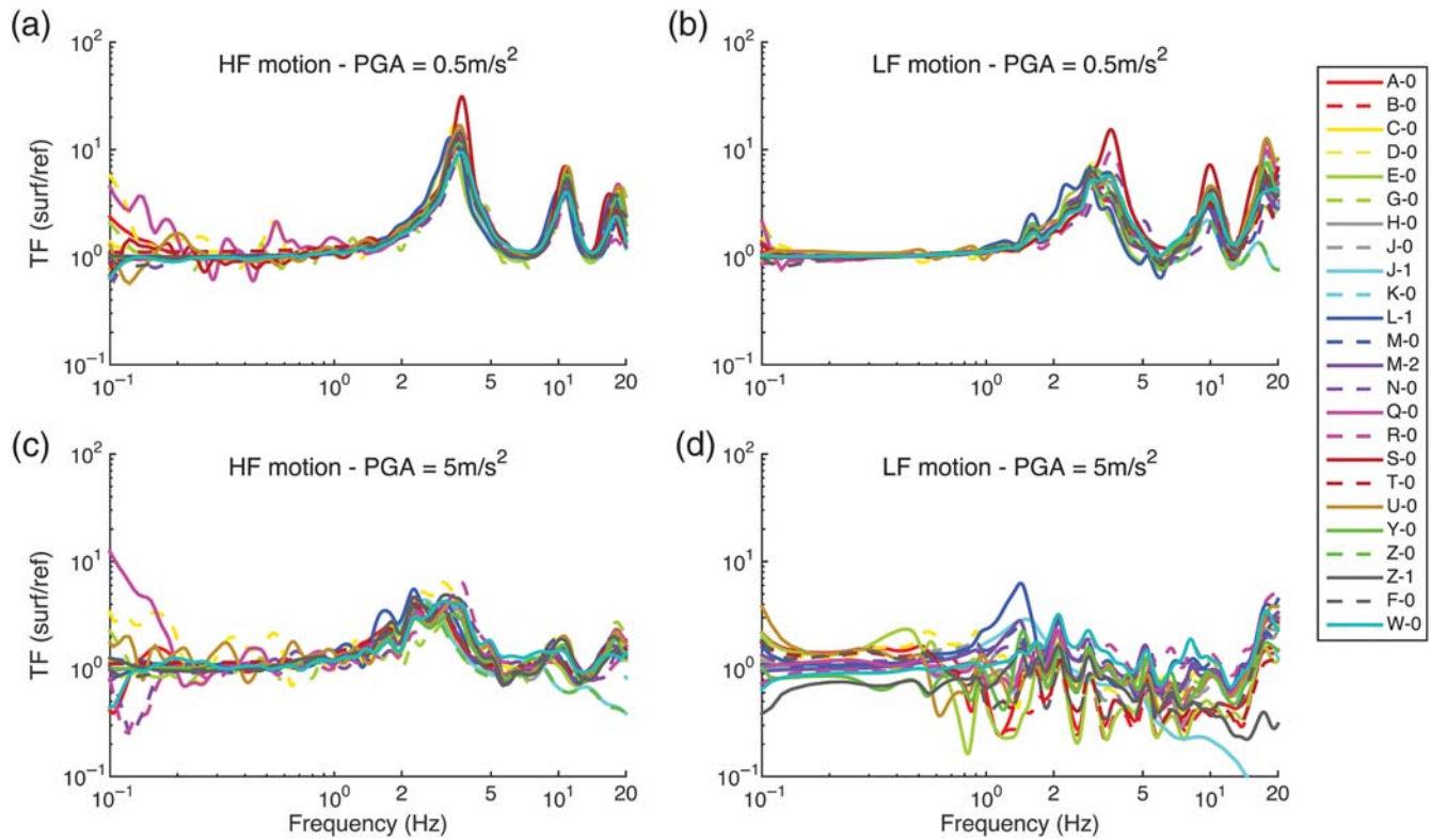
Figure 9. Comparison of the surface to reference Fourier spectra ratio, for the nonlinear (NL) computations using the HF input motion (a) scaled to 0.5 \text{ m/s}^2 and (c) scaled at 5 \text{ m/s}^2 , and using the LF input motion (b) scaled to 0.5 \text{ m/s}^2 and (d) scaled at 5 \text{ m/s}^2 .
