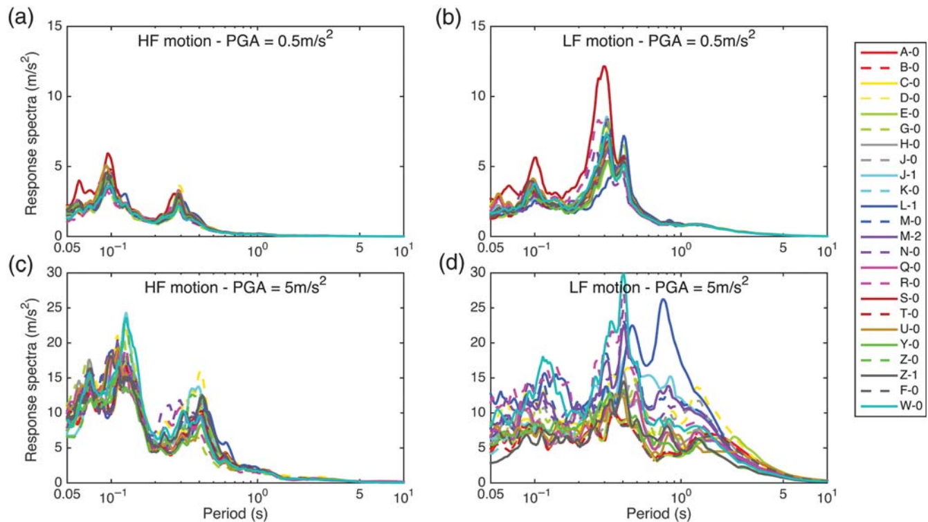
Figure 10. Comparison of the acceleration pseudoresponse spectra at the ground surface, for the NL computations using the HF input motion (a) scaled to 0.5 \text{ m/s}^2 and (c) scaled at 5 \text{ m/s}^2 , and using the LF input motion (b) scaled to 0.5 \text{ m/s}^2 and (d) scaled at 5 \text{ m/s}^2 .
