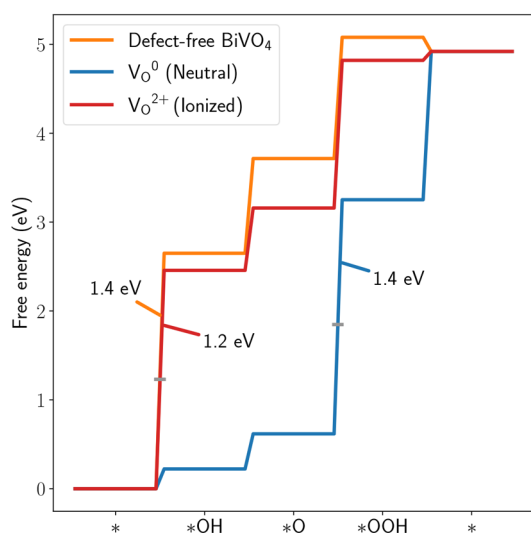
Figure 3. Free energy profiles for the OER as shown in eq 1 on stoichiometric as well as oxygen-deficient BiVO 4 , with the latter shown in both neutral (0) and ionized (+2) charge states. The location of the ideal barrier height for each PDS is marked with a horizontal bar, and the excess barrier energy is also shown. These result in overpotentials of 1.4 V for the stoichiometric surface, 1.4 V for V O 0 , and 1.2 V for the ionized V O 2+ .
