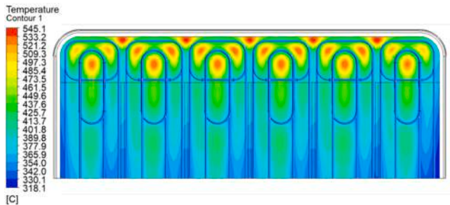
Fig. 4. Section of the outboard equatorial BU thermal field during DEMO operations, showing the arrangement of the BZ helicoidal-shaped DWTs cooling system [14].
