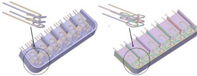
Fig. 3. Inboard (left) and outboard (right) BU with helicoidal-shaped DWTs.
