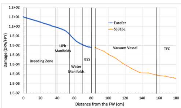
Fig. 18. Radial profile of the damage on Eurofer (up to the BSS) and SS-316, evaluated in the inboard BU.
