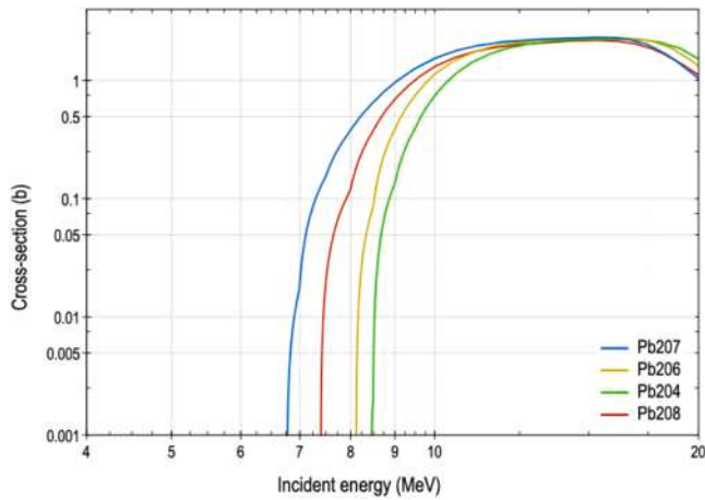
Fig. 23. Pb(n,n) reaction cross section (JEFF 3.3 nuclear data library [18]).
