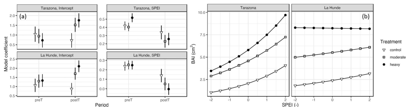
Fig. 3. Model coefficients for the fixed effects (mean values and 95% confidence intervals) for basal area increment (BAI) in Tarazona and La Hundé, for three treatment levels during pre-thinning ( preT ) and post-thinning ( postT ) periods (a), and generalized linear models of BAI against SPEI for different treatment levels in the postT period (b).
