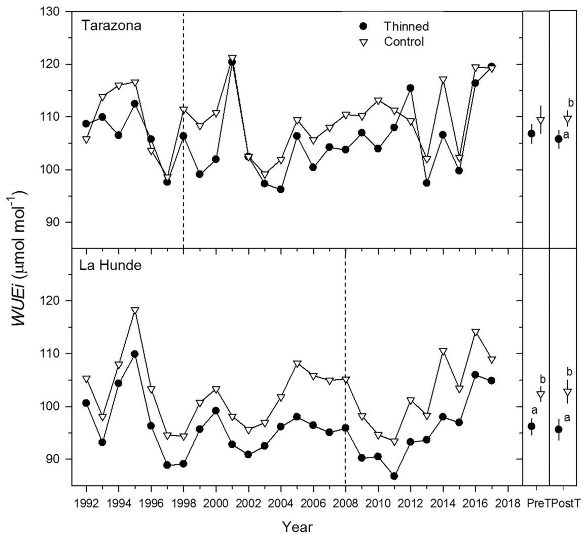
Fig. 5. Time series of the intrinsic water-use efficiency (WUEi) at Tarazona and La Hundo according to thinning treatments: control (empty triangles) and heavy thinning (filled dots). In both cases, n = 5 trees per treatment. Vertical dashed lines indicate the date of thinning treatments (1998 in Tarazona and 2008 in La Hundo). Right margin plots show mean and standard errors for both treatments during pre- ( preT ) and post-thinning ( postT ) periods, with significant ( p -value < 0.05) differences among treatments during each period indicated with letters.
