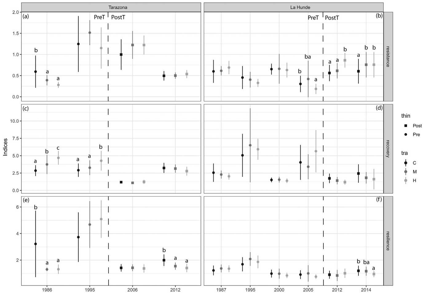
Fig. 4. Temporal evolution of tree resistance (a, b), recovery (c, d) and resilience (e, f) indices in response to selected droughts calculated for Tarazona (left panels) and La Hundo (right panels) growth data (BAI) considering control plots (C), moderately (M) and heavily thinned (H) plots. Values are shown before (circles, Pre) and after thinning (squares, Post) treatments. Vertical dashed lines indicate the date of thinning treatments. Bars represent standard deviations. Significant differences among thinning treatments are indicated with letters ( p -value < 0.05).
