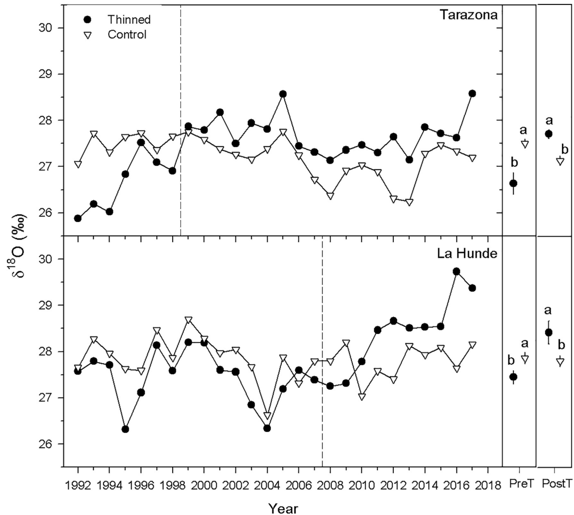
Fig. 7. Time series of \delta^{18}\text{O} values at Tarazona and La Hundo according to thinning treatments: control (empty triangles) and heavy thinning (filled dots). In both cases, n = 5 trees per treatment. Vertical dashed lines indicate the date of thinning treatments, and margin plots show the mean and standard deviation for each treatment during pre- ( preT ) and post-thinning ( postT ) periods, with significant ( p\text{-value} < 0.05 ) differences among treatments during each period indicated with letters.
