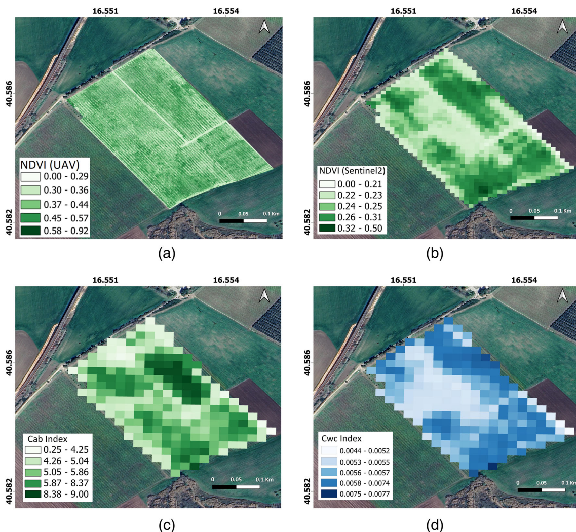
FIGURE 7 Input parameters of remote sensing images acquired on 2024 May the 28. (a) NDVI map from UAV (5 cm spatial resolution); (b) NDVI from Sentinel2 (10 m spatial resolution); (c) Canopy Chlorophyll Content Index computed from Sentinel2; (d) Canopy Water Content Index computed from Sentinel2.
