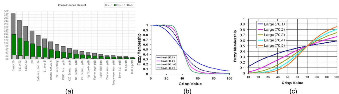
FIGURE 10 (a) Consolidates results, (b) Small and (c) Large membership function.
