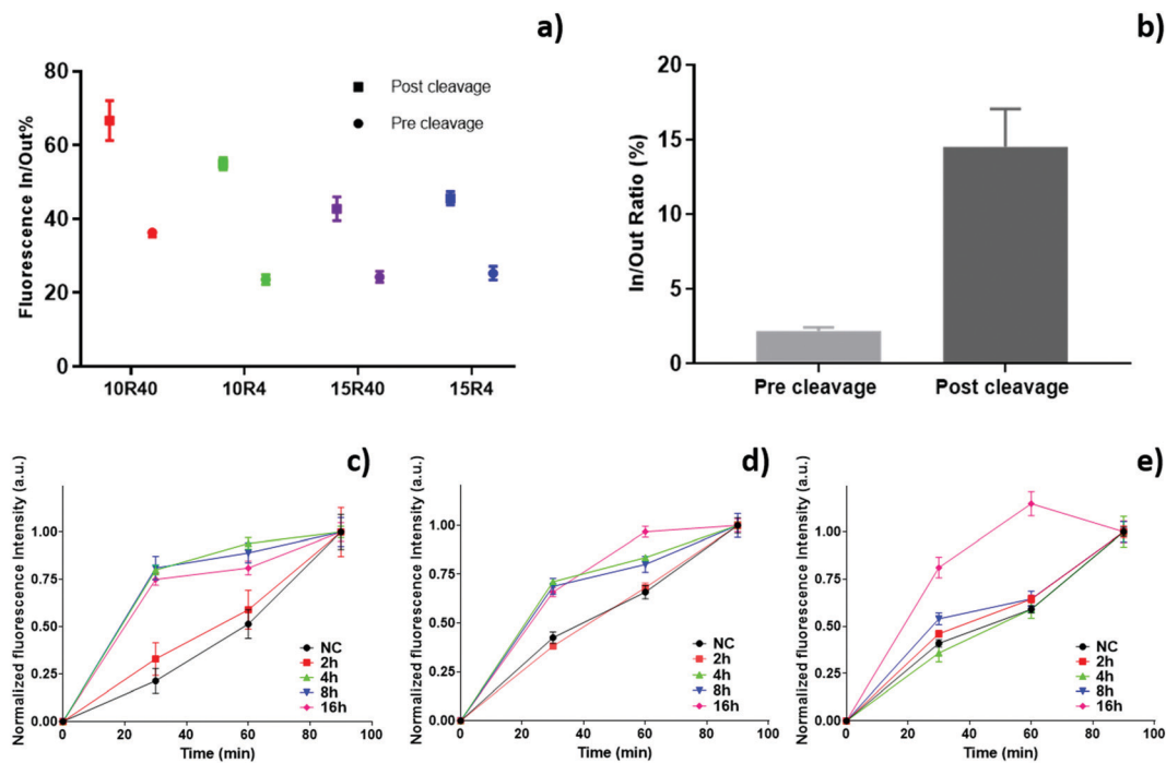
Fig. 3 (a) Fluorescence partition coefficient at equilibrium (120 min) for the diffusion of a labelled IgG inside the hydrogel microparticles, before and after the cleavage; (b) fluorescence partition coefficient at equilibrium (120 min) for the diffusion of labelled silica nanoparticles (diameter 50 nm) inside the 10R40 hydrogel microparticles, before and after the cleavage; Diffusion kinetics of fluorescent probes: (c) 17nt-oligonucleotide, (d) ovalbumin and (e) IgG performed on 10R40 microparticles with different cleavage times (non cleaved = NC, 2 h, 4 h, 8 h and 16 h cleaved MPs).
