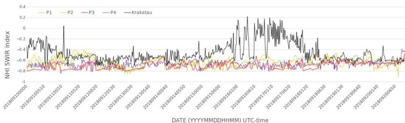
Figure 6. Time series of the NHI_{SWIR} index computed, from Himawari-8 AHI data of Figure 5b, over the Krakatau (black curve) and four background pixels (from P1 to P4) located far from the volcano (see Figure 5a). Note that values of the index higher than -0.4 were recorded only at Krakatau, in the presence of a documented lava effusion.
