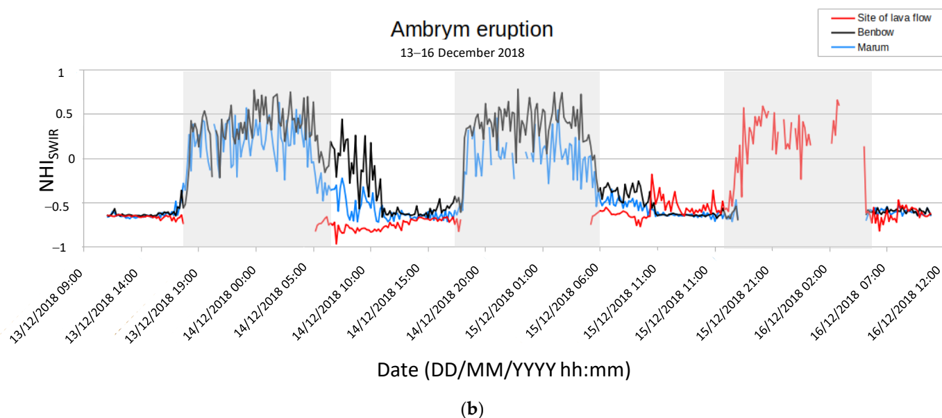
Figure 2. (a) Pixel boxes centred over Benbow (area #1), Marum (area #2) and SE flank of the Marum crater (area #3); (b) Time series of the NHI_{SWIR} index retrieved over the period 13 December 2018 at 09:00 LT–16 December 2018 at 11:00 LT, night-time intervals (17:00–06:00 LT) are marked in light grey. Note that the index was not calculated in the presence of low SWIR radiance values recorded at night-time for the reasons discussed in the text (see red curve; area #3).
