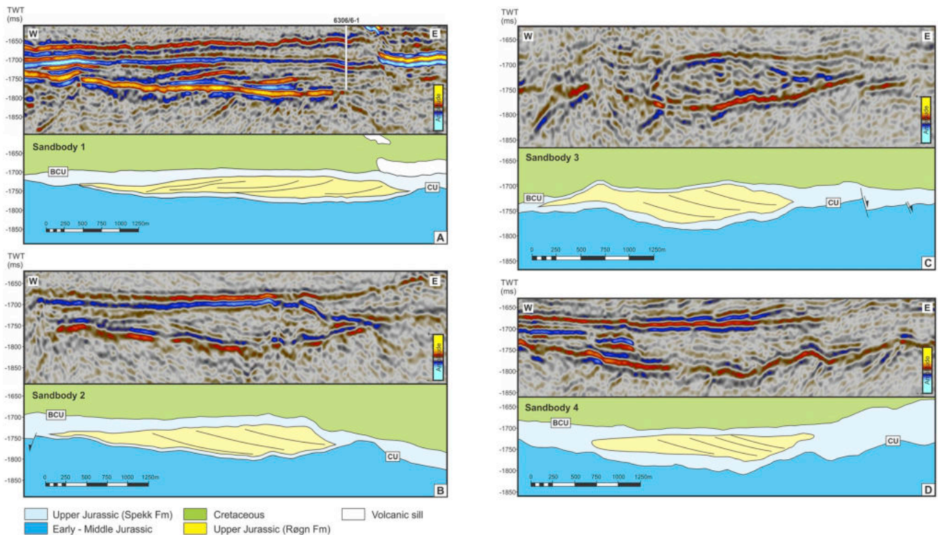
Fig. 5. Cross-sections of the recognised Upper Jurassic Rogn Fm sandbody showing their external lenticular shape encased within the Spekk Fm deposits. Sandbodies are internally characterised by westward (A) or eastward (B, C, and D) dipping reflectors indicating the lateral migration of the sand ridges during their evolution.
