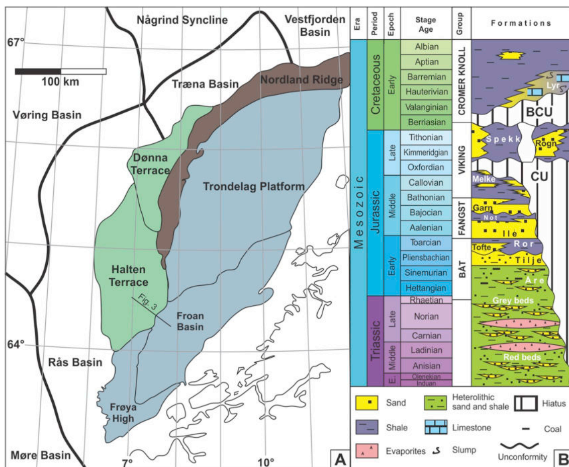
Fig. 1. A) Map of the main structural elements defined in the Haltenbanken area (modified after Blystad et al., 1995). (B) Stratigraphic column for the Mid-Norwegian shelf (based upon Dalland et al., 1988) highlighting the Triassic to Early Cretaceous stratigraphy. BCU: Base Cretaceous Unconformity; CU: Callovian Unconformity.
