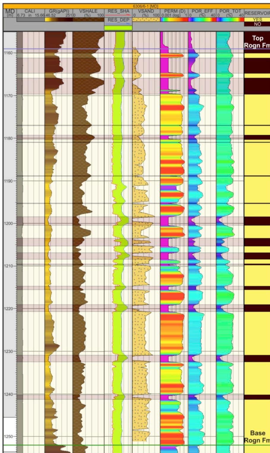
Fig. 13. Set of wireline logs for the well 6306/6-1 showing the main properties and patterns in the Rogn Fm interval (Frøya High).
