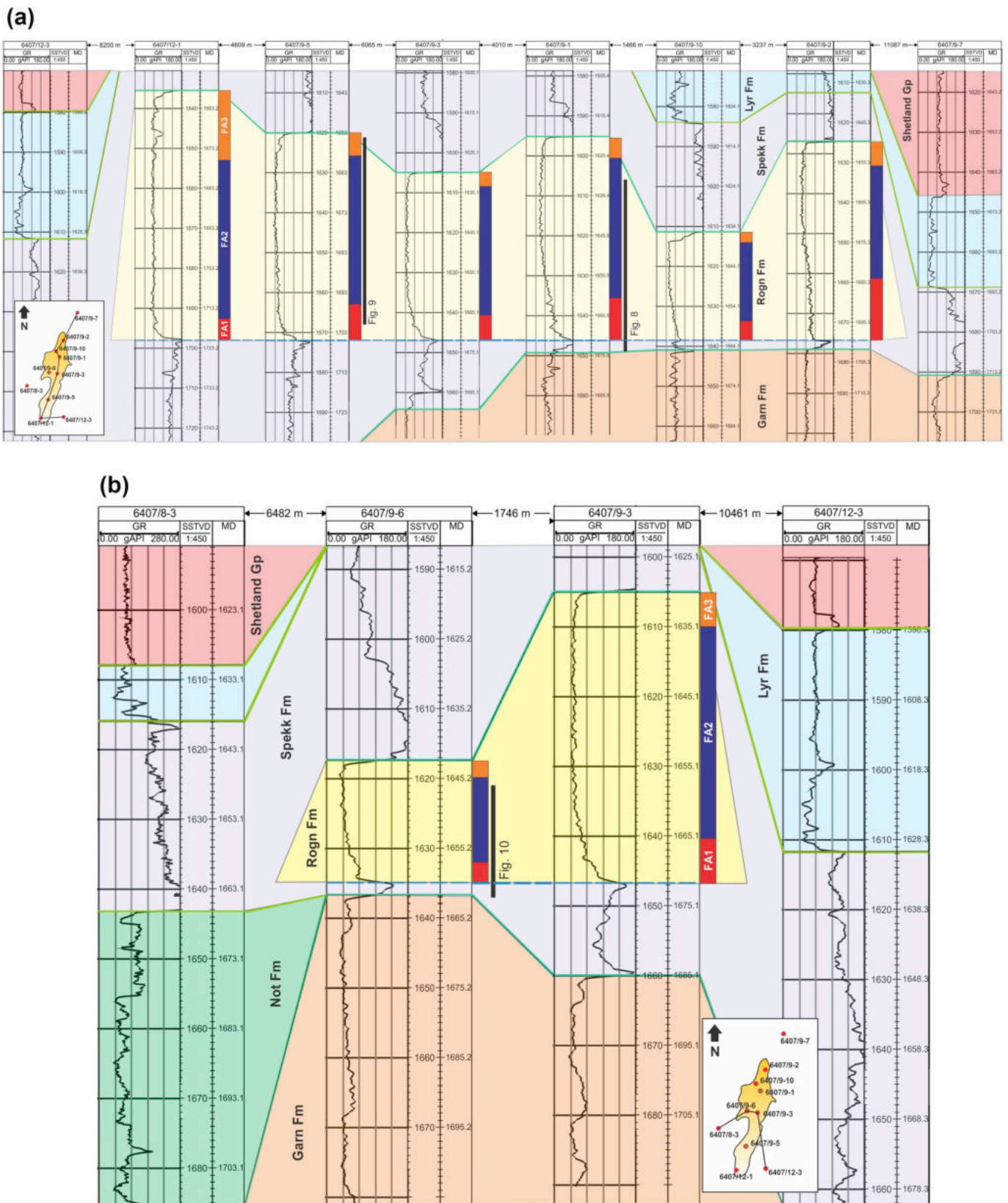
Fig. 6. (A) Correlation panel over the Draugen Field (Froan Basin) with north-south (A) and east-west (B) orientations. Black bars indicate the extent of core intervals.
