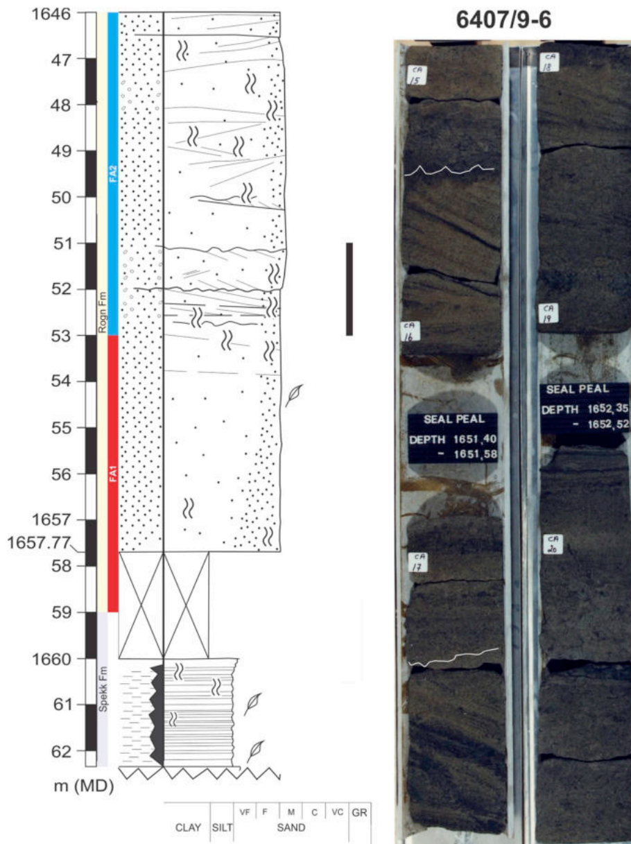
Fig. 10. Core log of the Rogn Fm from well 6407/9-6 showing medium- to coarse-grained sandstones organised into cross-strata. See Fig. 1 for location and Fig. 11 for the key.
