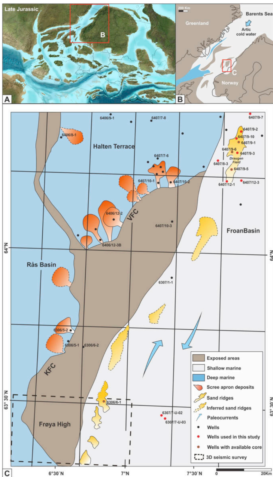
Fig. 2. A) Global palaeogeographic reconstruction of the northern Hemisphere in the Late Jurassic period 150 Ma. (Deep Time Maps™) B) Schematic reconstruction of the seaway between Norway and Greenland in the Late Jurassic, based on plate tectonic reconstructions by Ziegler (1988) and Dorè (1992). C) Reconstruction of a portion of the Norwegian Sea during the Late Jurassic (Kimmeridgian) across the Froan, Halten and Rås basins, and the Frøya High with used wells, and outline of seismic data used. Scree apron deposits located along the Klakk Fault Complex (KFC) and Vingleia Fault Complex (VFC), and shallow marine sand ridges accumulated in the Trøndelag Platform (i.e. Froan Basin and Frøya High) are represented.
