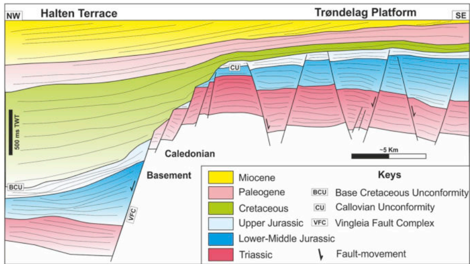
Fig. 3. Schematic cross-section over the Halten Terrace and the Trøndelag Platform. See Fig. 2 for orientation.
