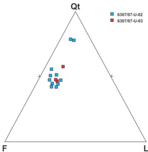
Fig. 12. Ternary diagram showing the petrographic composition of the Rogn Fm in the wells 6307/07-U-02 and 6307/07-U-03. Results show a general quartz-feldspathic composition.
