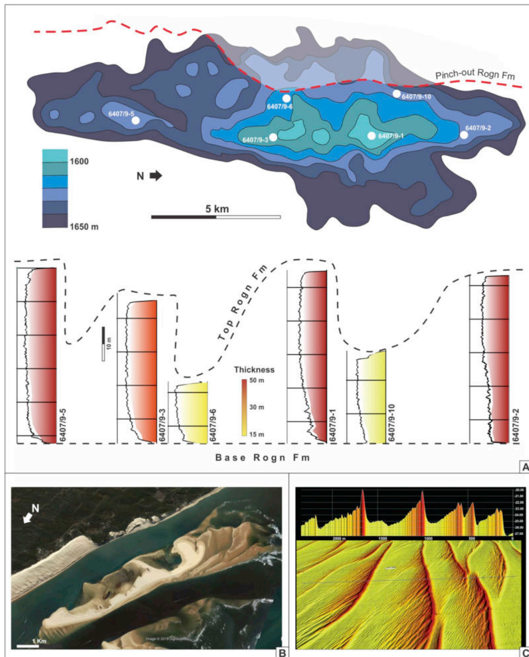
Fig. 14. –A) Depth map of the Top Rogn reservoir (Draugen Field) highlighting the lenticular shape of the sandbody as recognised in the Frøya High area (see Fig. 5), and N-S profile along the Draugen sand ridge. B) Satellite image of a modern sand ridge (Banc d'Arquin, France) showing plan view geometry comparable with what recognised in the Draugen Field and bedforms 1–4. C) Bathymetric profile and multibeam echosounder bathymetry of tidal bedforms (Breaksea Shoa, Australia) showing the typical vertical profile along a sand ridge. 3D image of a 150 m long nuclear submarine is shown for scale (Image courtesy of Ron Boyd).
