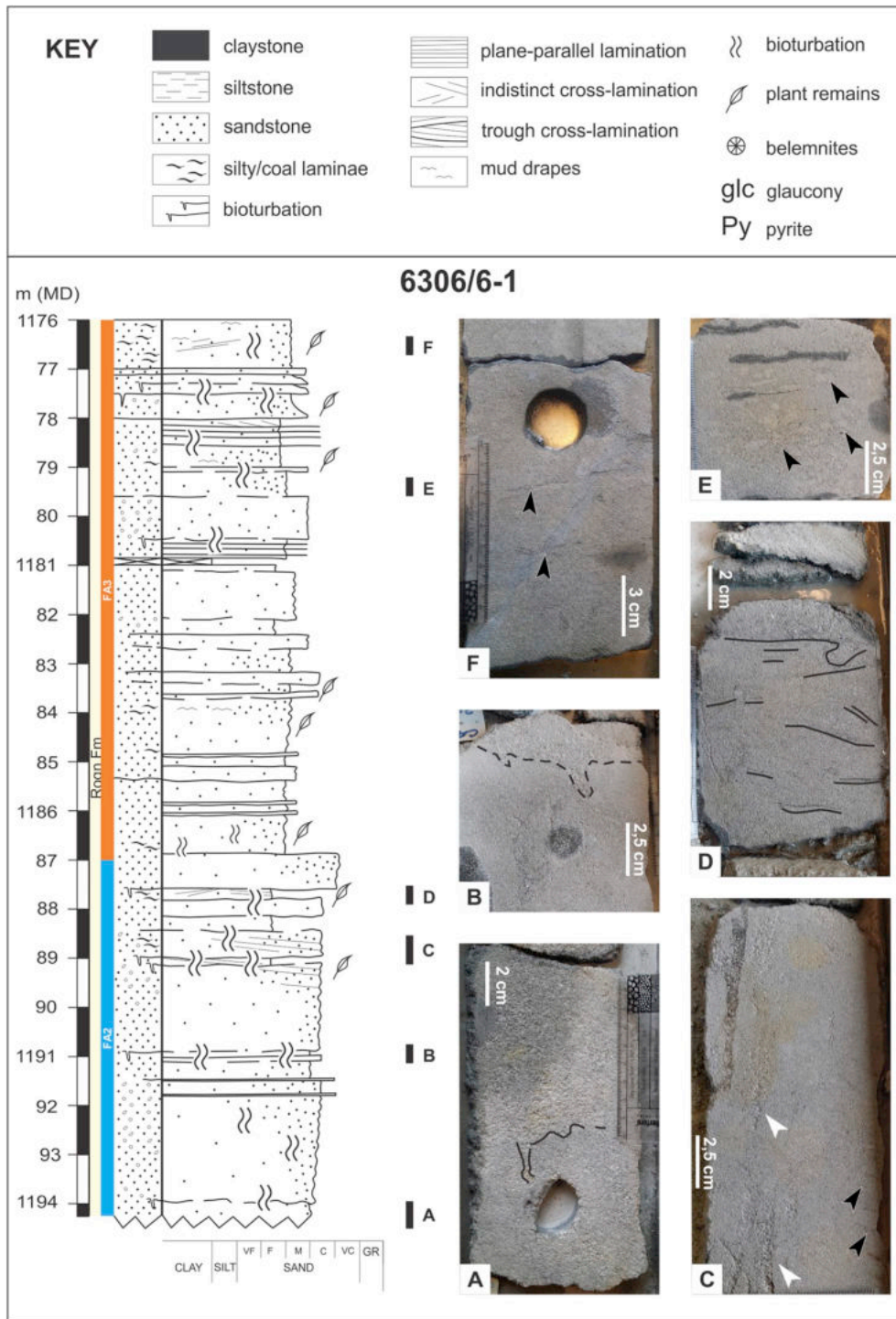
Fig. 11. Core log of the Rogn Fm from well 6306/6-1. A, B and D) Sharp contact between medium-grained and coarse-grained sandstone. The boundary is characterised by the presence of vertical bioturbations. C) Coarse-grained sandstones showing indistinct inclined cross-lamination highlighted by silty laminae (black arrows) and vertical trace-fossils. E) Fine- to medium-grained sandstones showing horizontal trace-fossils. F) Fine- to medium-grained sandstones with indistinct inclined lamination highlighted by silty laminae (black arrows). See Fig. 1 for location.
